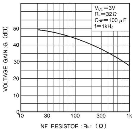
Fig. 13 Voltage gain vs. feedback resistor value
