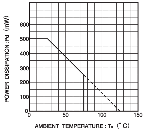
Fig. 16 Thermal derating curve
