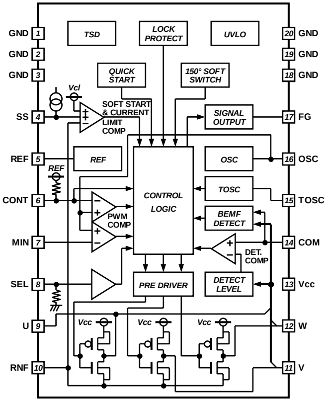
Fig. 2 Block diagram
