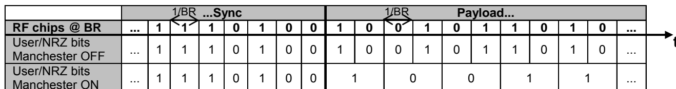
Figure 46: Manchester Encoding/Decoding
