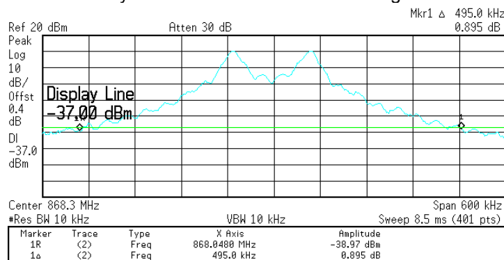
Figure 83: FSK - 25 kbps - +/-50 kHz
