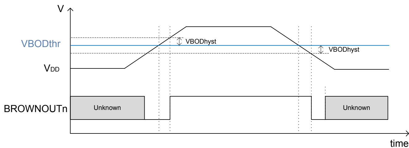
Figure 9.3. RMU Brown-out Detector Operation
