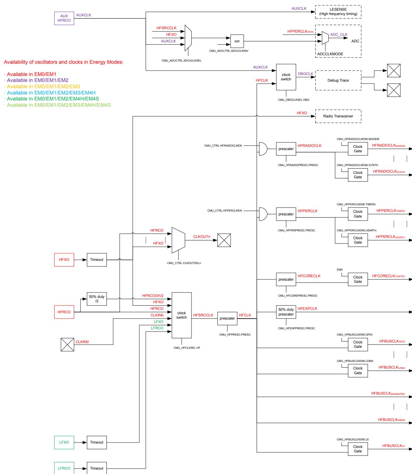
Figure 11.1. CMU Overview - High Frequency Portion
