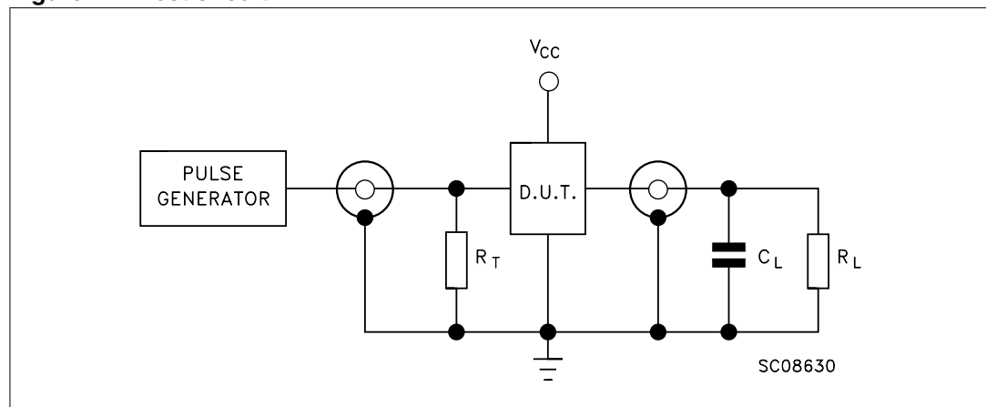
Figure 4. Test circuit
