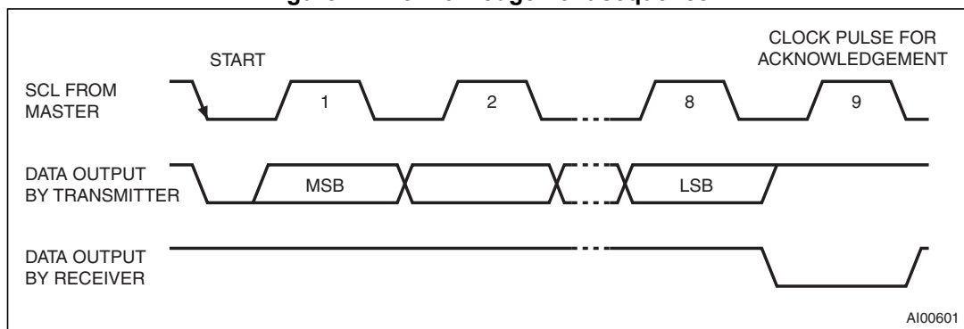
Figure 11. Acknowledgement sequence
