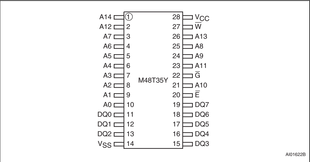
Figure 3. SOIC connections
