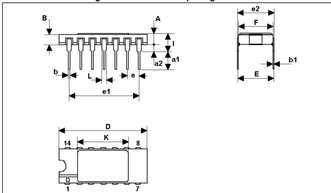
Figure 3. Ceramic DIL-14 package outline
