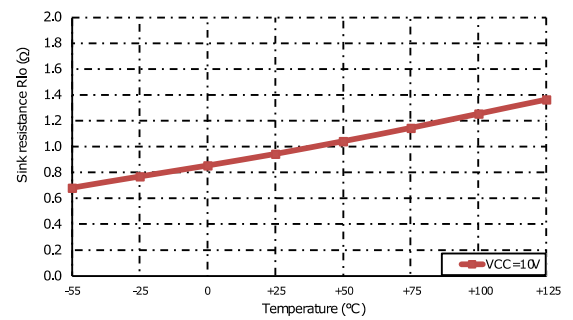
Figure 21: Sink resistance vs temperature
