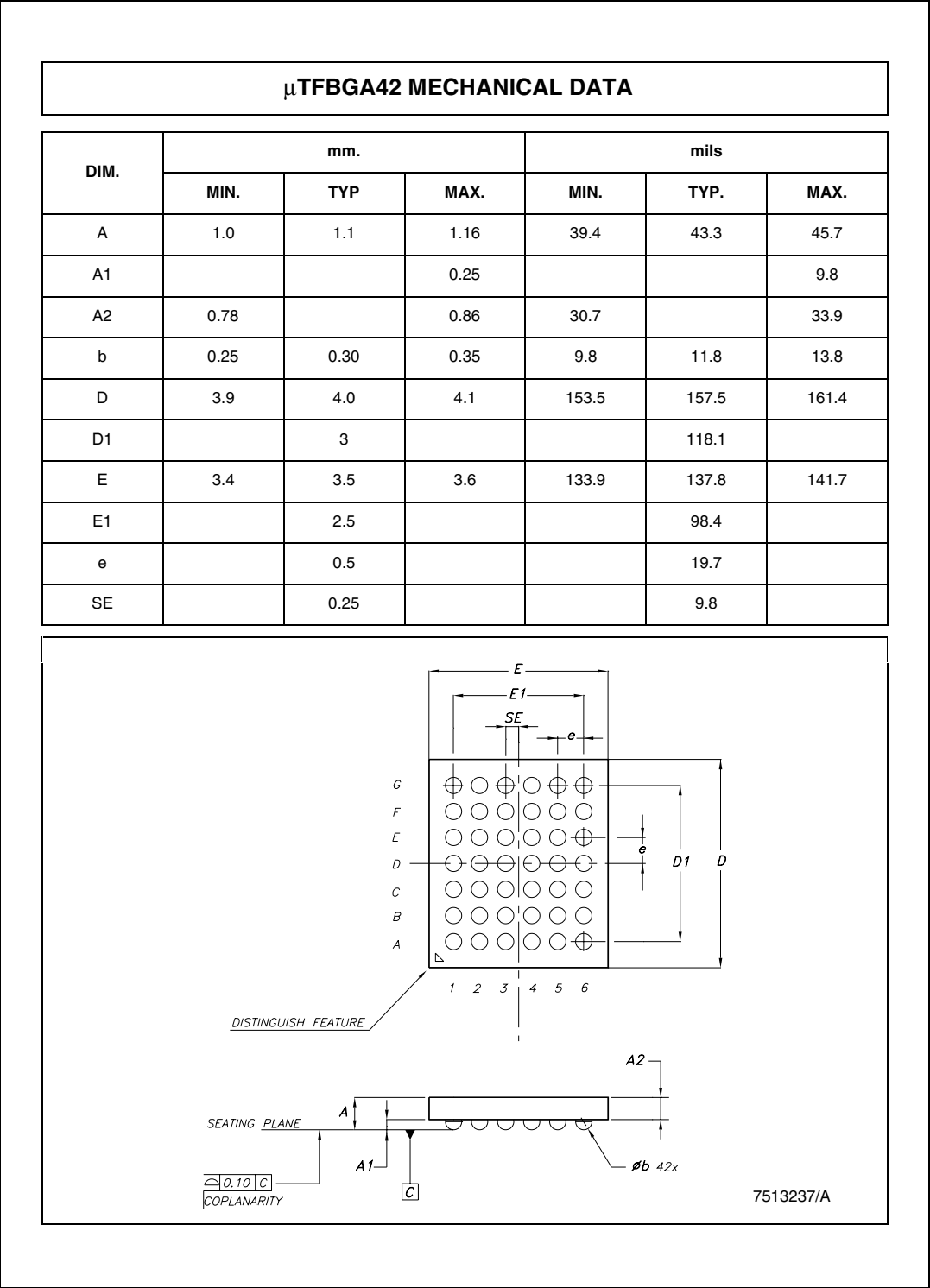
Figure 8. \mu TFBGA42 mechanical data
