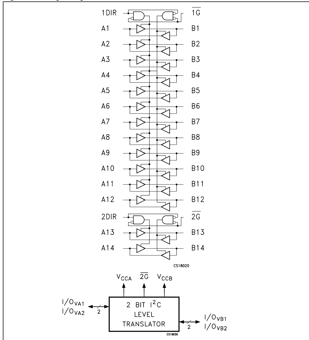
Figure 1. Logic diagram
