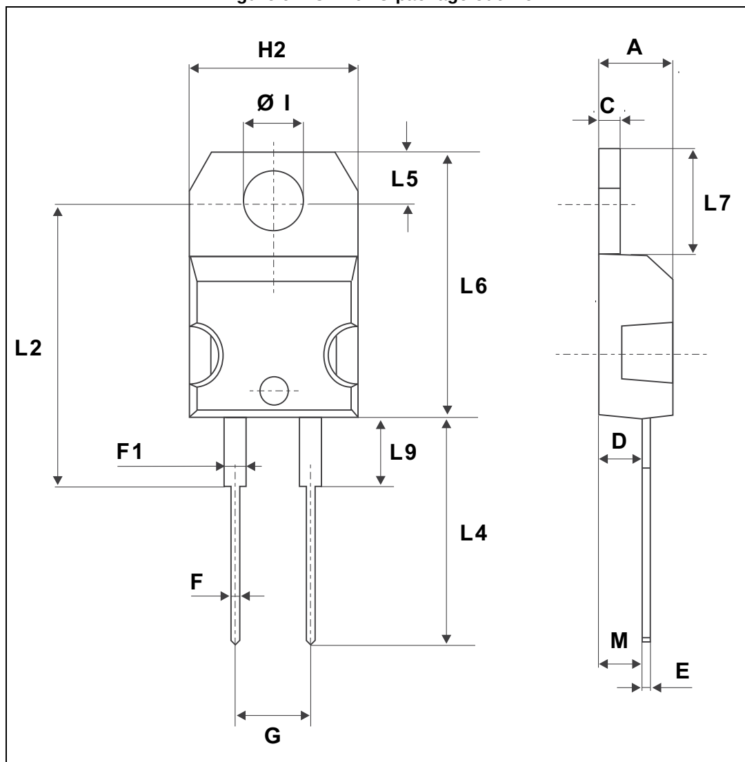
Figure 9. TO-220AC package outline
