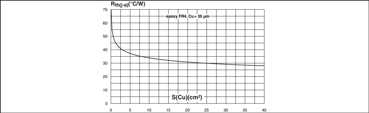
Figure 13. Thermal resistance junction to ambient versus copper surface under tab (D 2 PAK)
