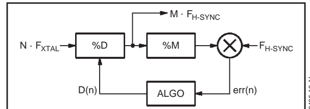
Figure 10 : Digital PLL
