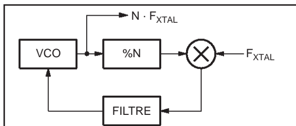
Figure 9 : Analogic PLL
