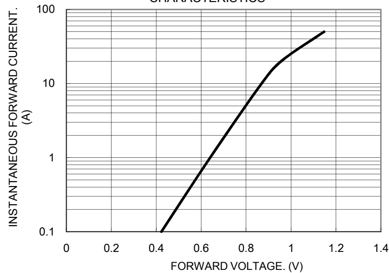
FIG. 4- TYPICAL INSTANEOUS FORWARD CHARACTERISTICS
