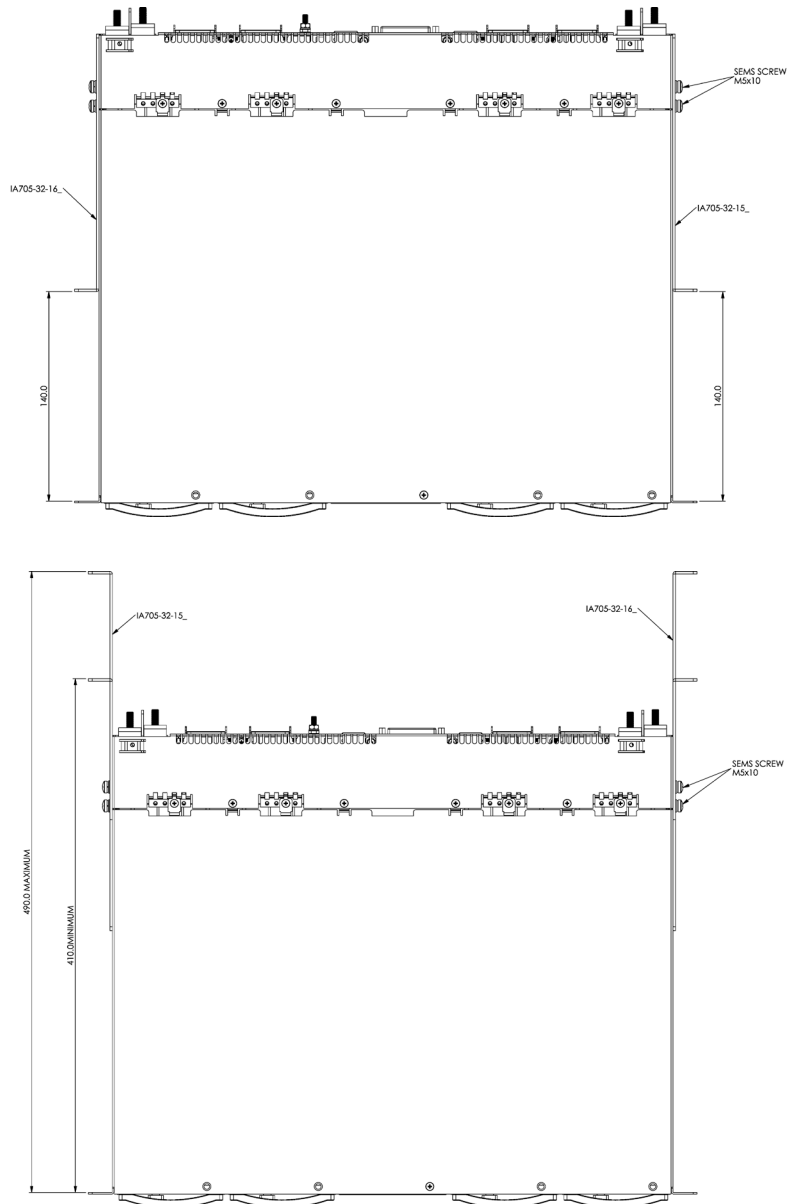
Fig 2.5 Mounting options, brackets and screws are included.
