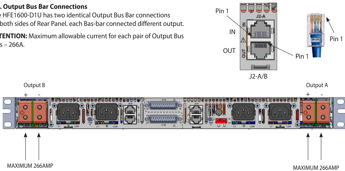
Fig 1.3a Output Bus-Bars.
