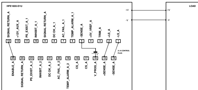
Fig 3.6 Output Voltage programming by External Voltage.
