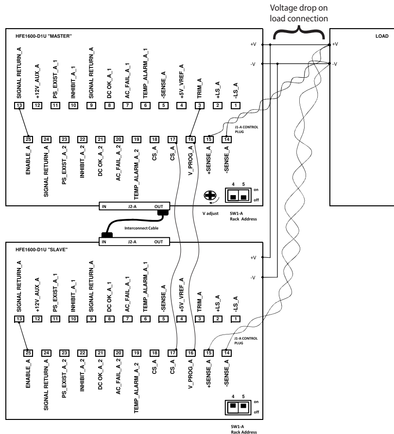
Fig 3.9 Racks parallel connection diagram.
