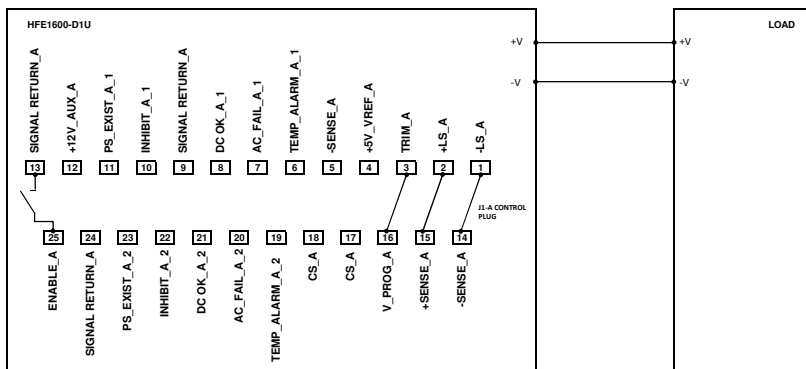
Fig 3.3 Entire rack On/Off control diagram.
