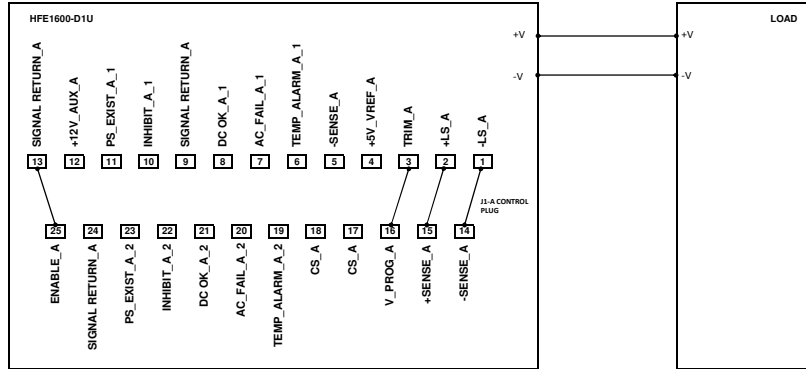
Fig 3.1 Basic connection diagram.
