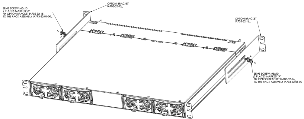
Fig 2.5 Mounting options, brackets and screws are included.
