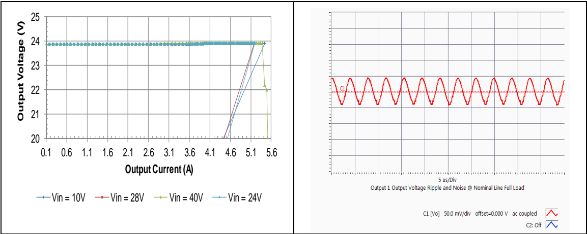
HQA2W085W240V Typical Output Current Limit Characteristics vs. Input Voltage at Ta=25 degrees
