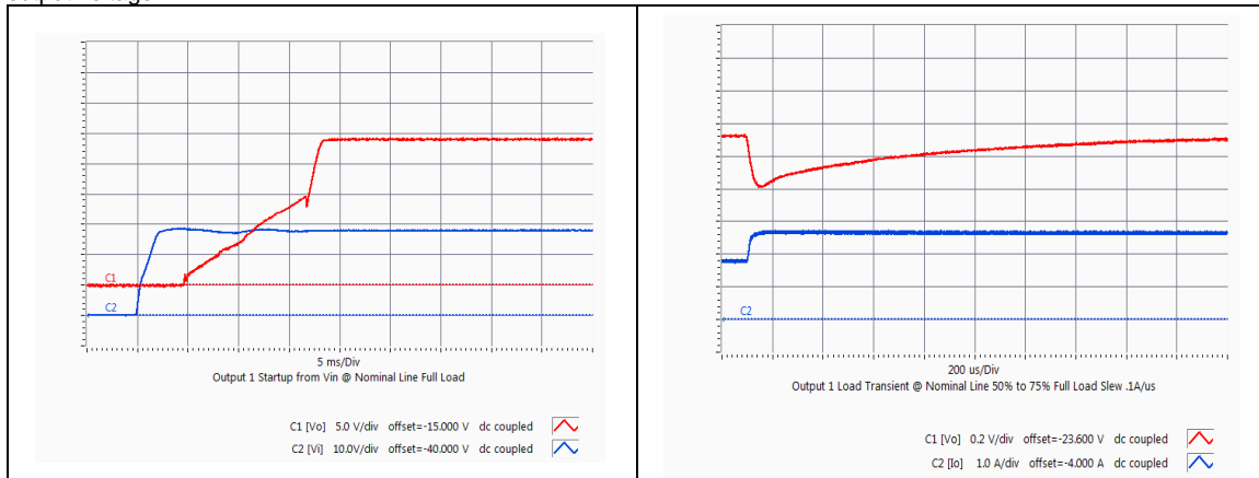
HQA2W085W240V Typical startup characteristic from input voltage application at full load. Red trace - output voltage, blue trace - input voltage
