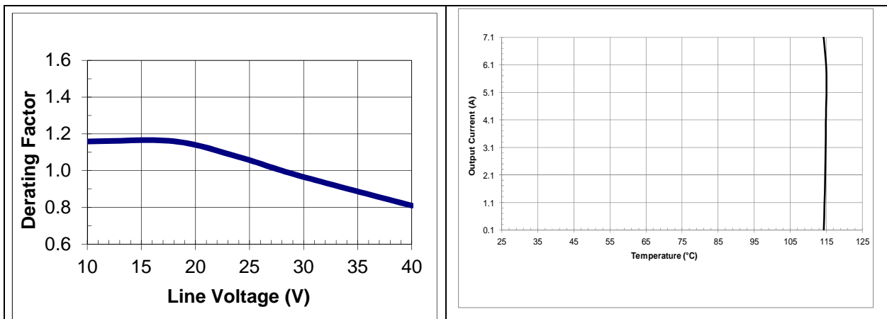
HQA2W085W2120V typical temperature derating versus input voltage output with 2m/s (400 lfm) airflow from pin 3 to pin 1
