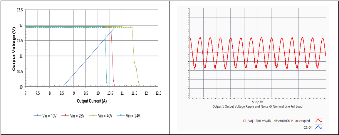
HQA2W085W120V Typical Output Current Limit Characteristics vs. Input Voltage at Ta=25 degrees
