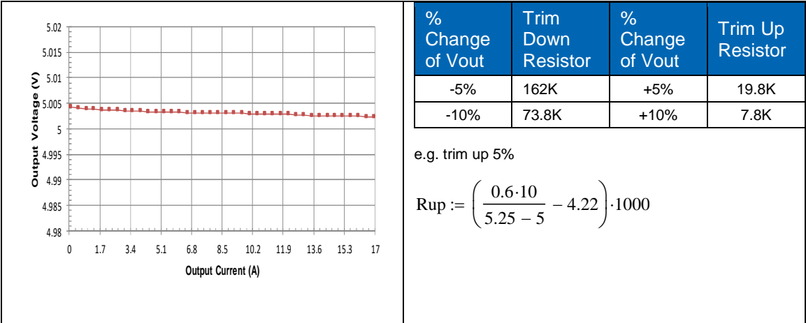
HQA2W085W050V Typical Load Regulation Characteristics at Ta=25 degrees
