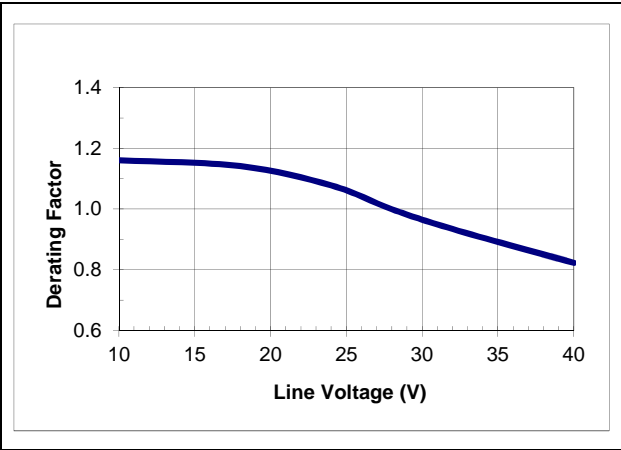
HQA2W085W150V typical temperature derating versus input voltage output with 2m/s (400 lfm) airflow from pin 3 to pin 1
