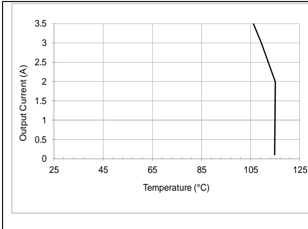
HQA2W085W240V maximum output current vs. baseplate temperature at nominal line
