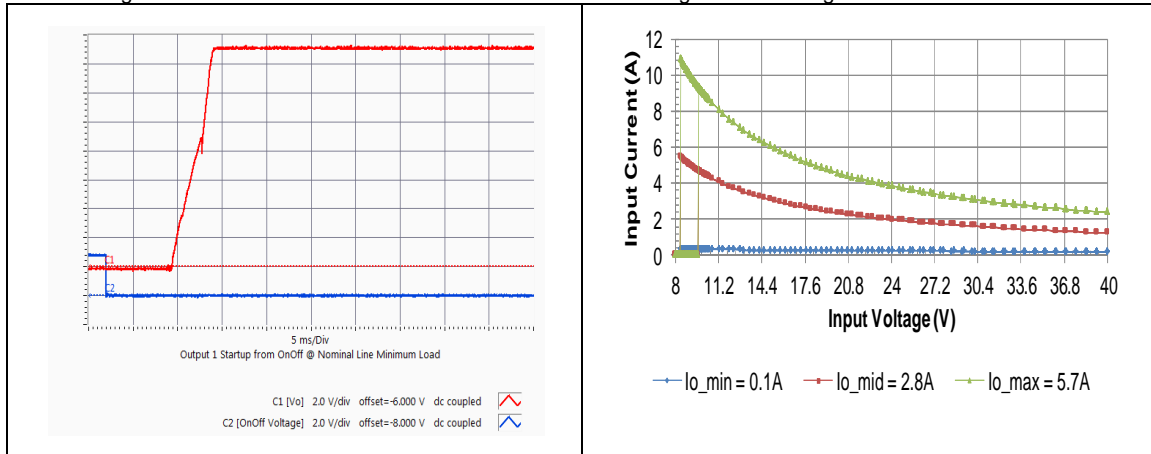
HQA2W085W150V Typical startup characteristic from on/off at light load. Lower trace - on/off signal, upper trace - output voltage
