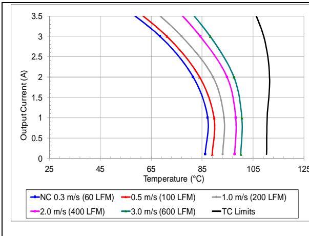
HQA2W085W240V maximum output current vs. ambient temperature at 28V input for airflow rates natural convection (60lfm) to 600lfm with airflow from pin 3 to pin 1
