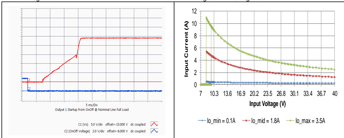
HQA2W085W240V Typical startup characteristic from on/off at full load. Blue trace - on/off signal, red trace - output voltage
