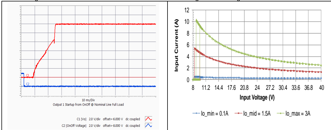
HQA2W085W280V Typical startup characteristic from on/off at full load. Blue trace - on/off signal, red trace - output voltage
