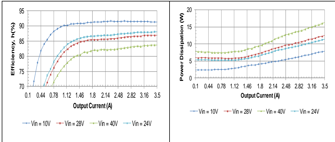
HQA2W085W240V Typical Efficiency vs. Input Voltage at T_a = 25 degrees
