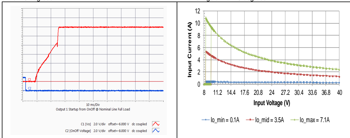
HQA2W085W120V Typical startup characteristic from on/off at full load. Lower trace - on/off signal, upper trace - output voltage
