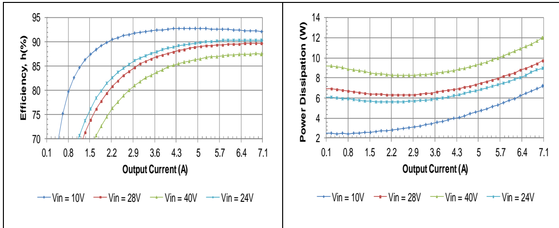
HQA2W085W120V Typical Efficiency vs. Input Voltage at T_a=25 degrees
