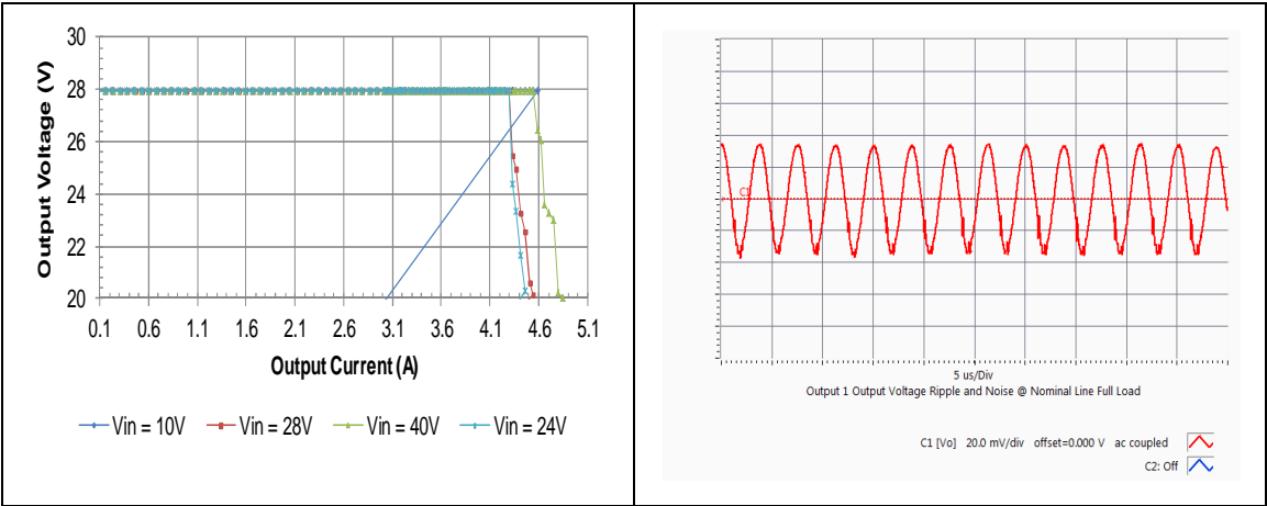
HQA2W085W280V Typical Output Current Limit Characteristics vs. Input Voltage at Ta=25 degrees
