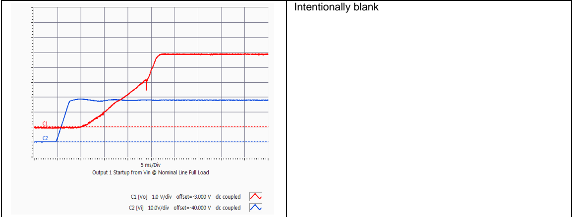
HQA2W085W050V Typical startup characteristic from input voltage application at full load. Red trace - output voltage, Blue trace - input voltage
