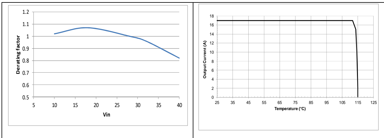
HQA2W085W050V typical temperature derating versus input voltage output with 2m/s (400 lfm) airflow from pin 3 to pin 1
