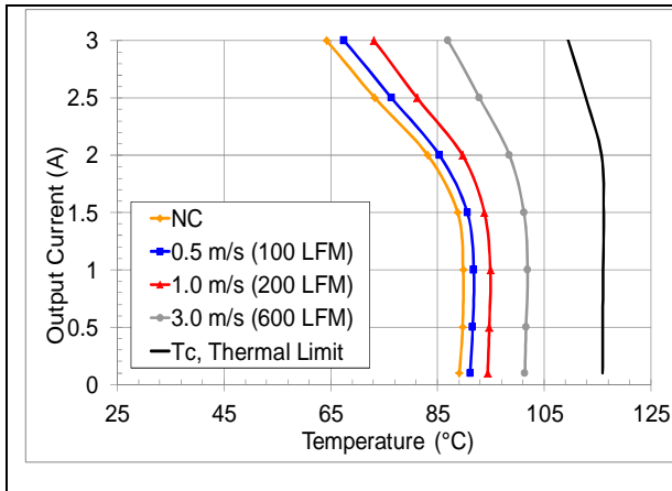
HQA2W085W280V maximum output current vs. ambient temperature at 28V input for airflow rates natural convection (60lfm) to 600lfm with airflow from pin 3 to pin 1
