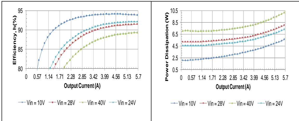
HQA2W085W150V Typical Efficiency vs. Input Voltage at T_a = 25 degrees
