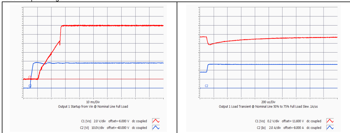
HQA2W085W120V Typical startup characteristic from input voltage application at full load. Red trace - output voltage, Blue trace - input voltage
