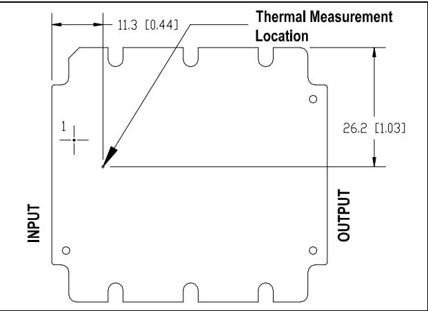
HQA2W085W150V thermal measurement location – top view
