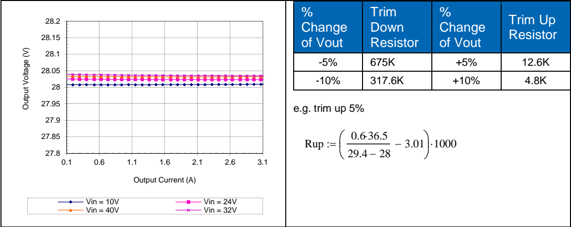
HQA2W085W280V Typical Load Regulation Characteristics at Ta=25 degrees
