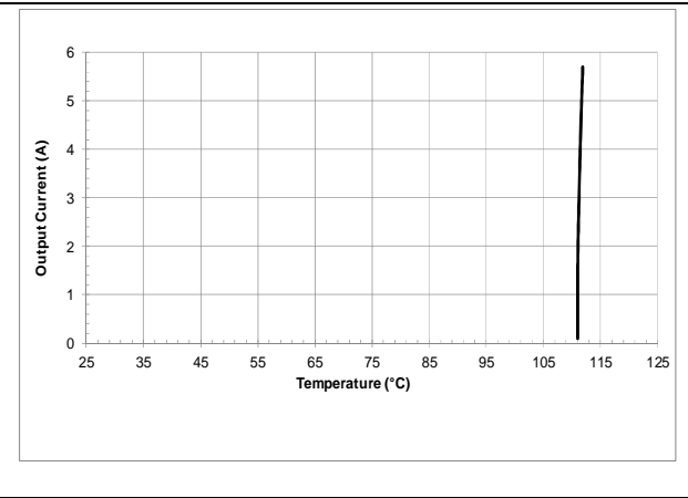
HQA2W085W150V maximum output current vs. baseplate temperature at nominal line
