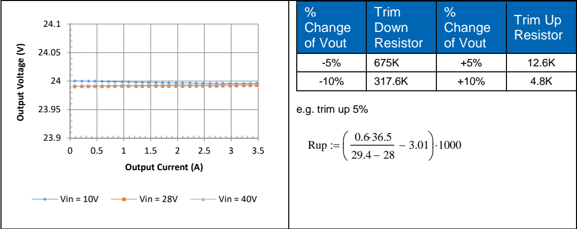
HQA2W085W240V Typical Load Regulation Characteristics at Ta=25 degrees
