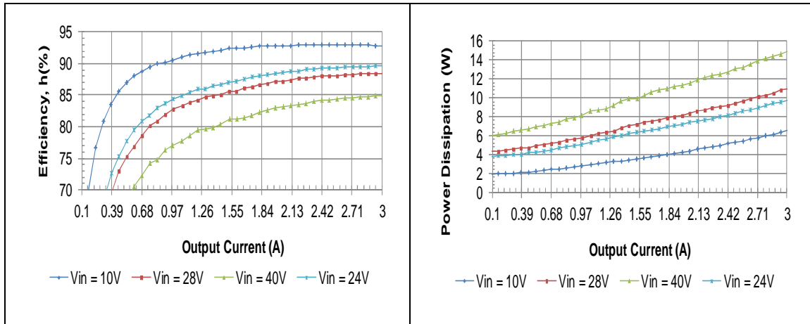
HQA2W085W280V Typical Efficiency vs. Input Voltage at T_a = 25^\circ\text{C}
