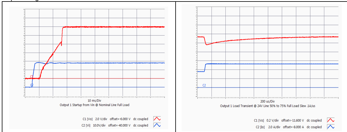
HQA2W085W280V Typical startup characteristic from input voltage application at full load. Red trace - output voltage, blue trace - input voltage
