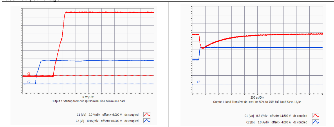
HQA2W085W150V Typical startup characteristic from input voltage application at light load. Red trace - output voltage, Blue trace - input voltage
