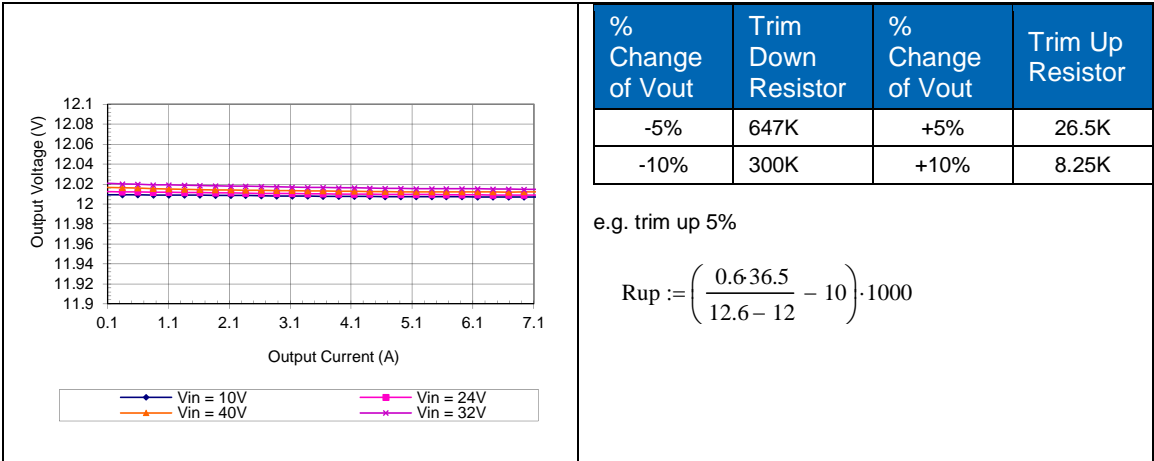
HQA2W085W120V Typical Load Regulation Characteristics at Ta=25 degrees
