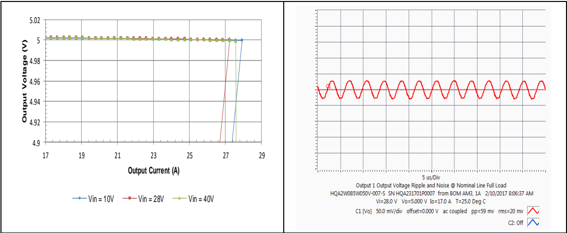
HQA2W085W050V Typical Output Current Limit Characteristics vs. Input Voltage at Ta=25 degrees
