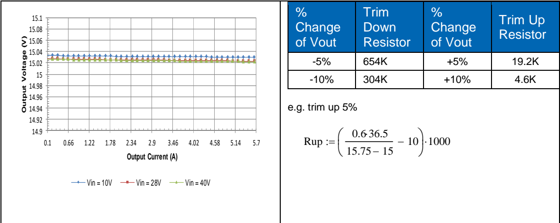
HQA2W085W150V Typical Load Regulation Characteristics at Ta=25 degrees
