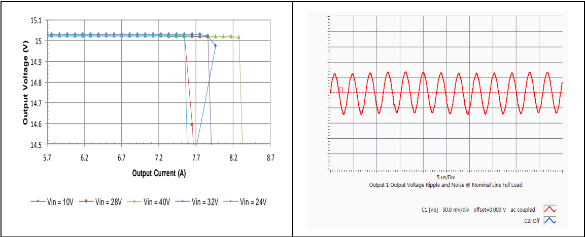
HQA2W085W150V Typical Output Current Limit Characteristics vs. Input Voltage at Ta=25 degrees
