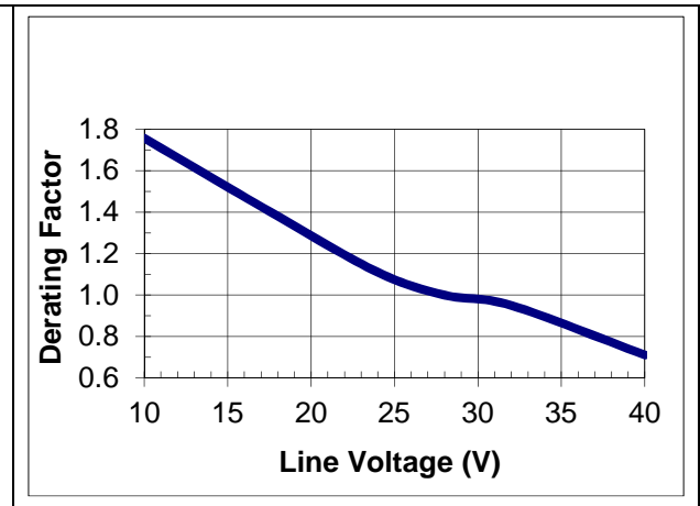
HQA2W085W240V typical temperature derating versus input voltage output with 2m/s (400 lfm) airflow from pin 3 to pin 1
