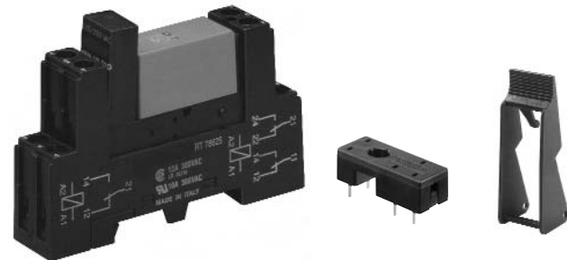
RT78625 with RPMU0730 RP78601 RT16016
