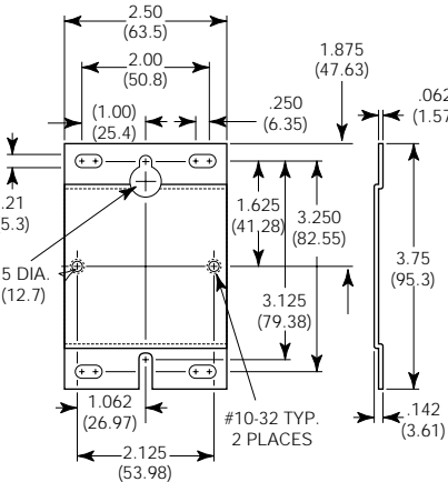
Mounting Plate Footprint
