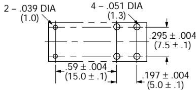
PC Board Layout (Bottom View)
