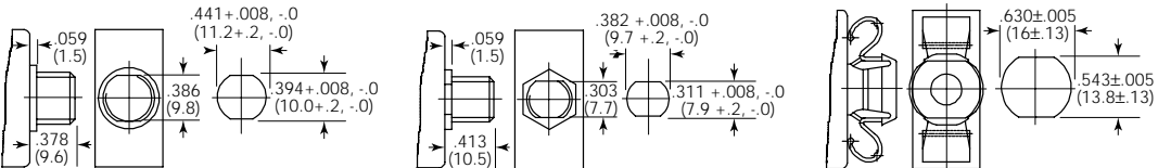
Special Order – M11 X 1.0 Thread Special Order – 3/8" - 24UNF Thread Special Order – Snap In Option
