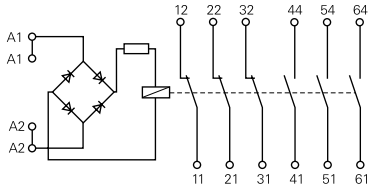
AC/DC Module, 3 NO + 3 NC
