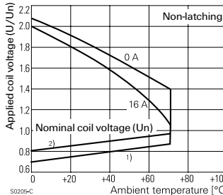
Non-Latching Models
