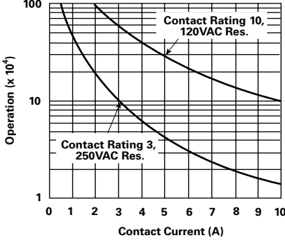
Life Expectancy
