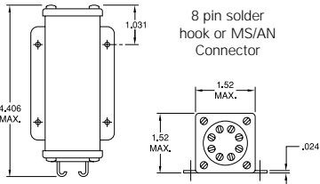
Panel Mount —9
