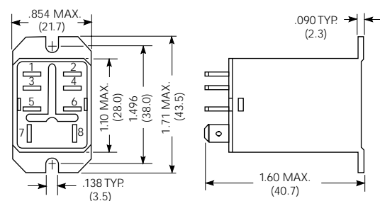
PCLH type (Flange Mount Case)
