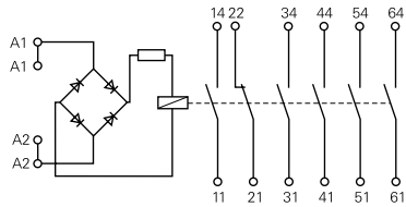
AC/DC Module, 5 NO + 1 NC
