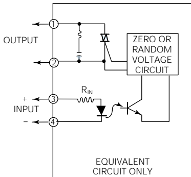
OAC Operating Diagram
