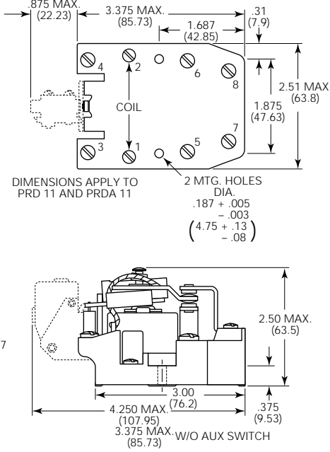
PRD/PRDA Large Base - Top View
