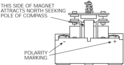
PRD3 with Magnetic Blow-Out
