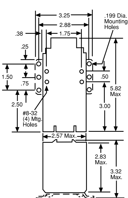
Models 7014, 7024
