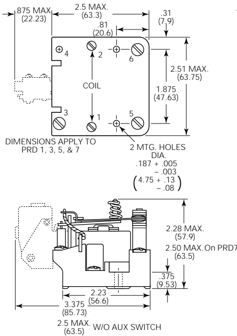
PRD/PRDA Small Base - Top View
