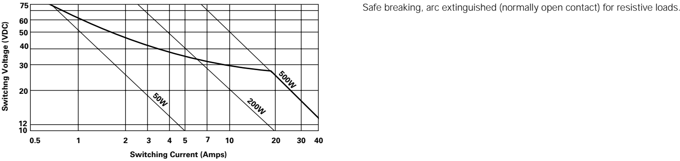
Figure 1 – Limiting Curve for Power Load
