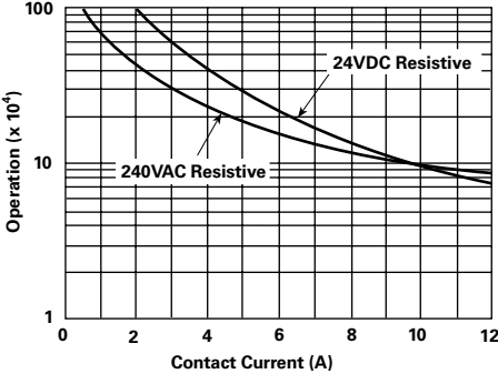
Life Expectancy
