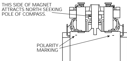
PRD11 with Magnetic Blow-Out
