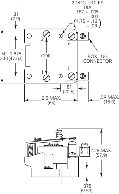
50 Amp PRD
