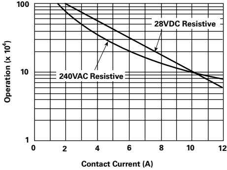
Life Expectancy
