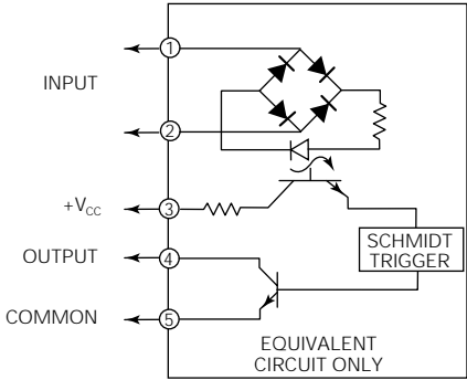
IAC Operating Diagram
