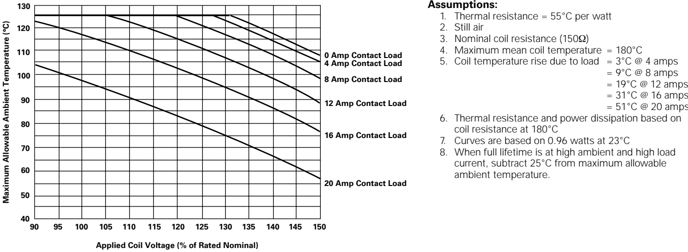
Figure 2 - Ambient Temperature vs. Coil Voltage for Continuous Duty
