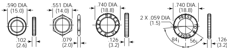
Standard Knurled Nut Standard Hex Nut Special Integrated Knurled Nut Special Integrated Knurled Nut with Small Holes
