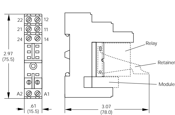
RP16104 Plastic Retaining Clip
