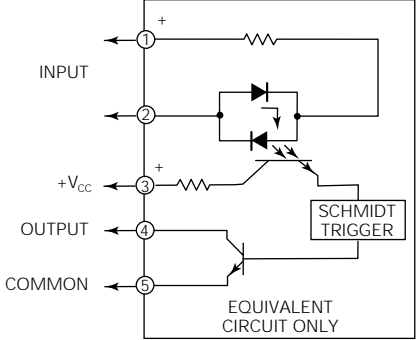
IDC Operating Diagram
