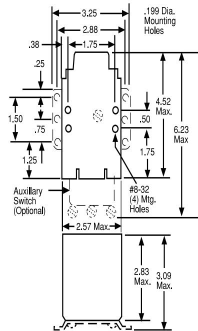
Models 7012, 7022
