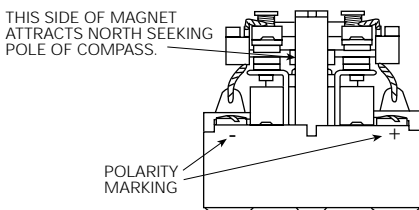
PRD7 with Magnetic Blow-Out
