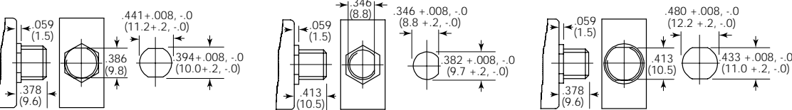
Standard Option 1 – M11 X 1.0 Thread Standard Option 2 & 6 – 3/8" - 24UNF Thread Standard Option 7 – M12 X 1.0 Thread
