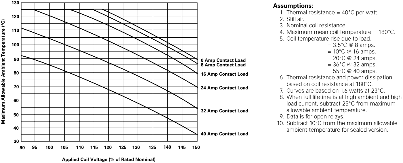
Figure 2 – Ambient Temperature vs. Coil Voltage for Continuous Duty
