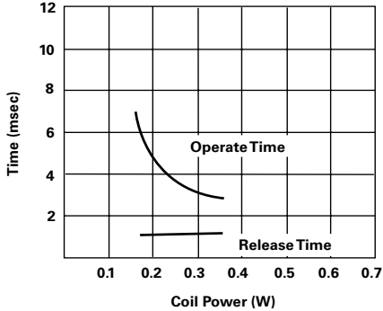
Operate Time
