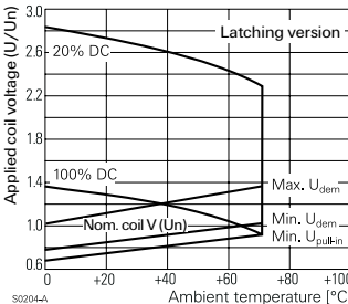
Latching Models
