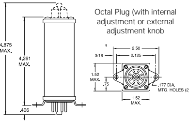
Chassis Mount —4, —5
