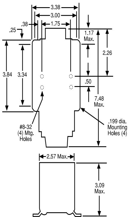
Model 7032
