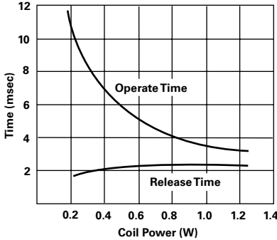
Operate Time
