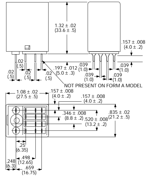
PCL 4c, 4a type (PCB Terminal)
