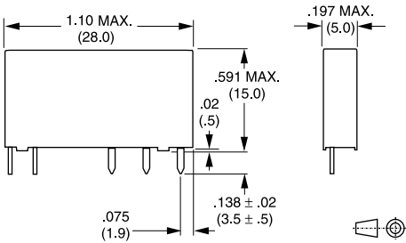
Vertical Version
