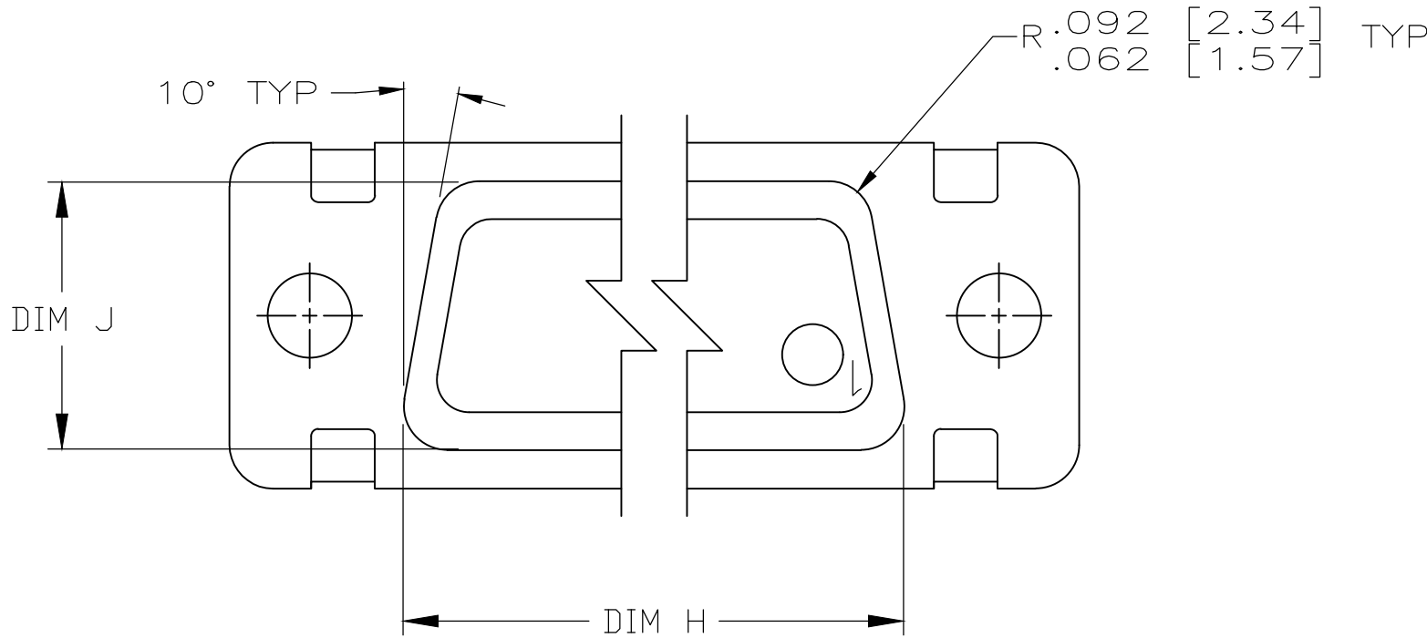
VIEW Z-Z
