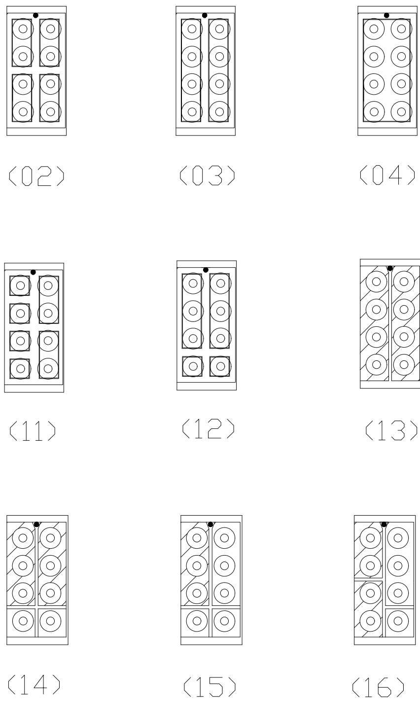
BUSSING ARRANGEMENT
