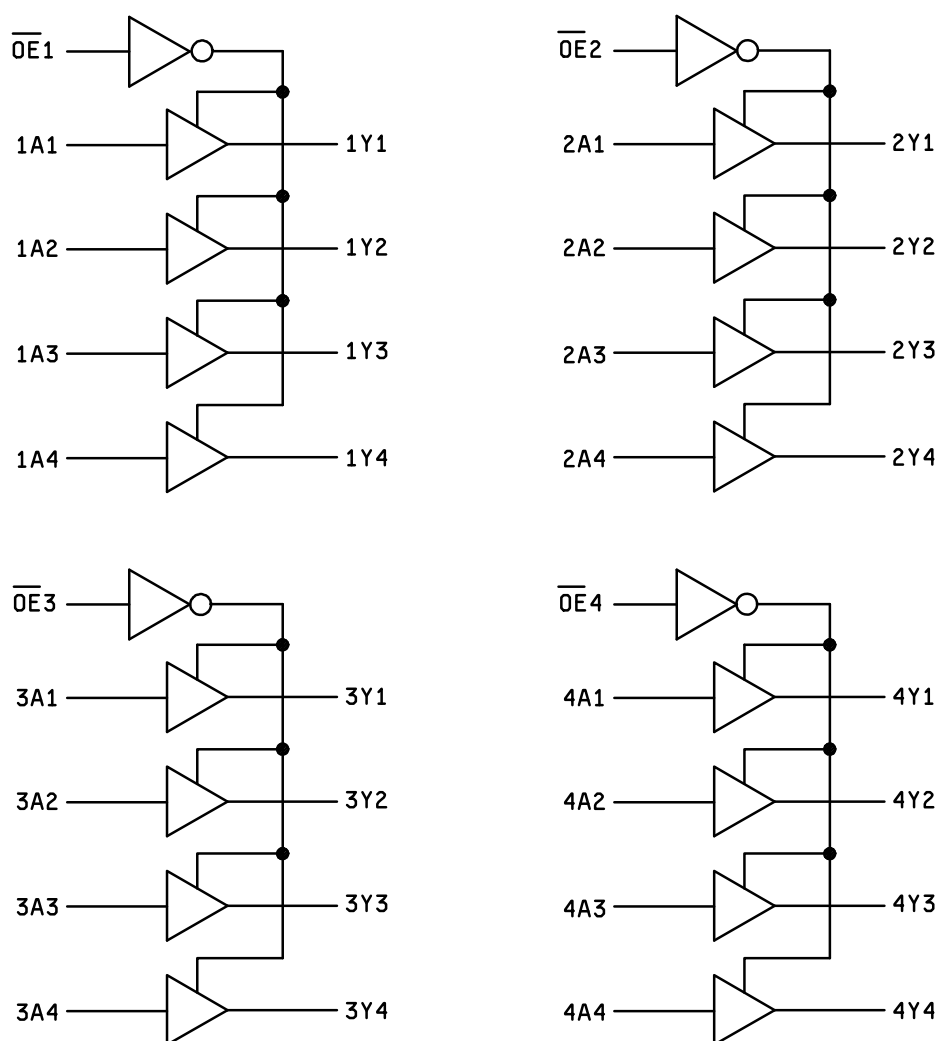
FIGURE 3. Logic diagram.
