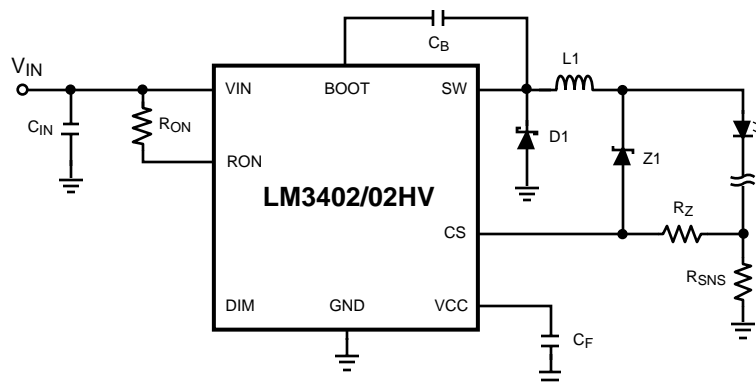
Figure 20. Output Open Circuit Protection
