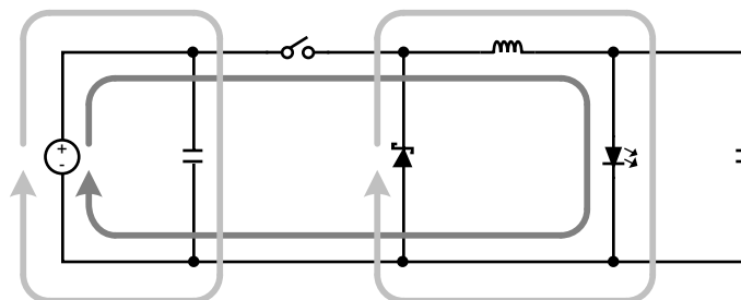
Figure 31. Buck Converter Current Loops
