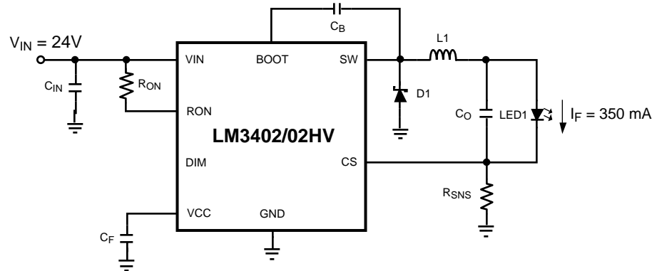
Figure 30. Schematic for Design Example 1
