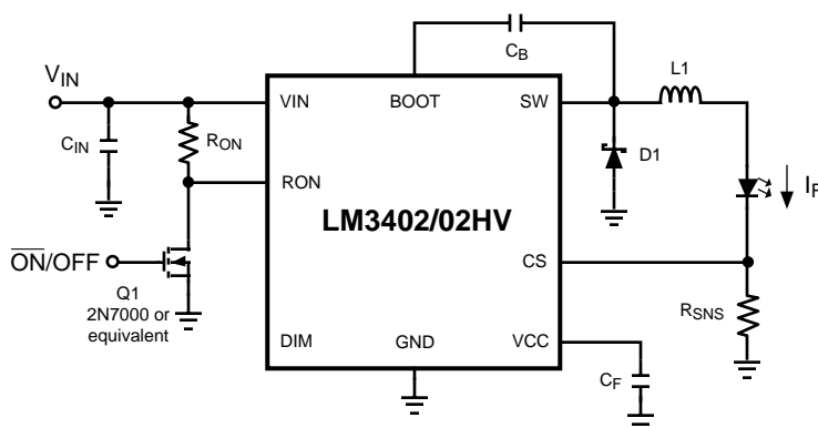
Figure 21. Low Power Shutdown
