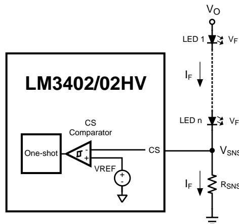
Figure 19. Comparator and One-Shot
