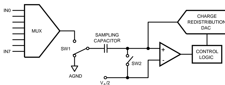
Figure 5. ADC128S022 in Hold Mode
