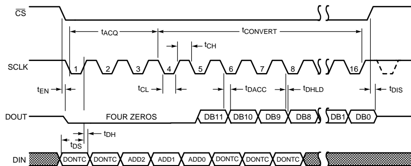
Figure 2. ADC128S022 Serial Timing Diagram
