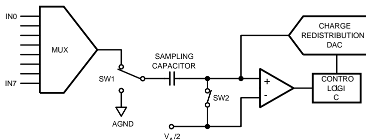
Figure 4. ADC128S022 in Track Mode
