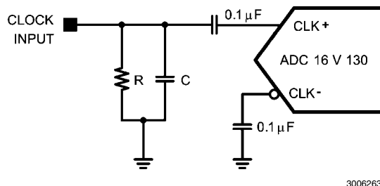
FIGURE 8. Singled-Ended 1.8V Clocking, Capacitive AC Coupled
