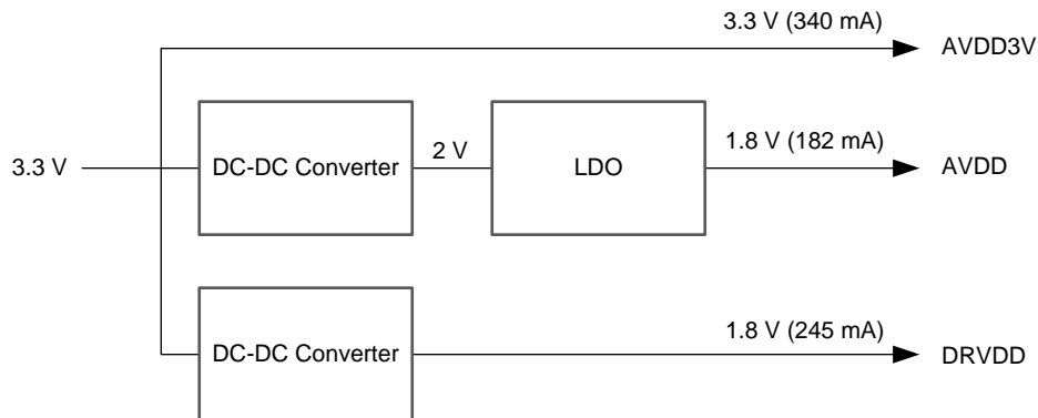
Figure 123. Example Power-Supply Scheme
