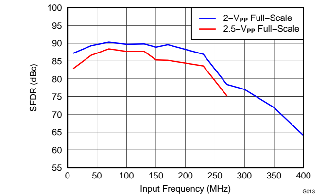
Figure 13. SFDR vs Input Frequency
