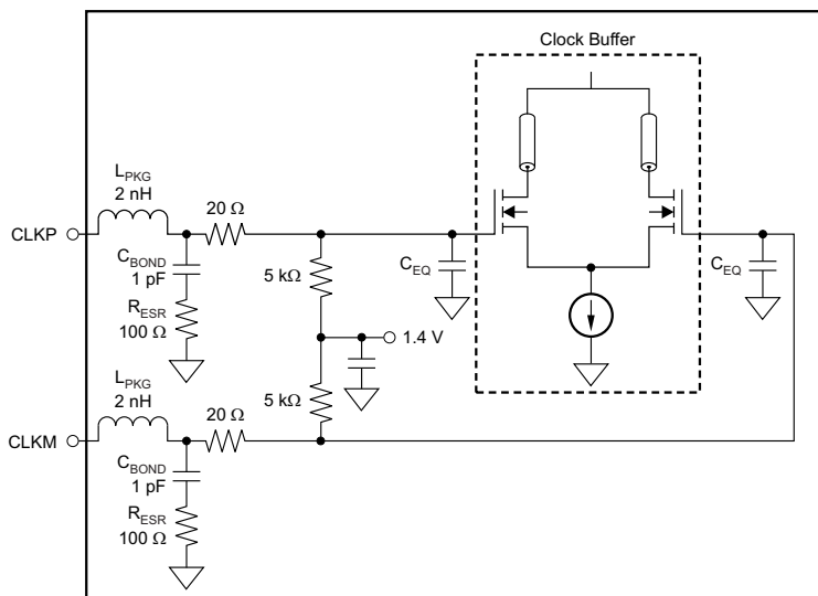
Figure 118. Internal Clock Buffer
