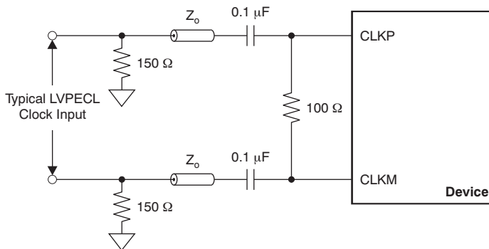
Figure 117. LVPECL Clock Driving Circuit
