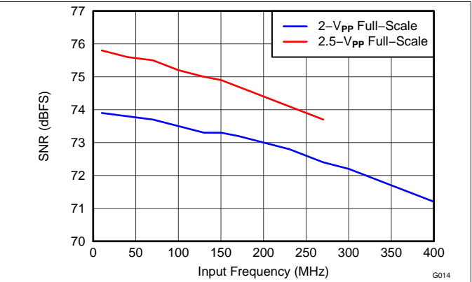
Figure 14. SNR vs Input Frequency
