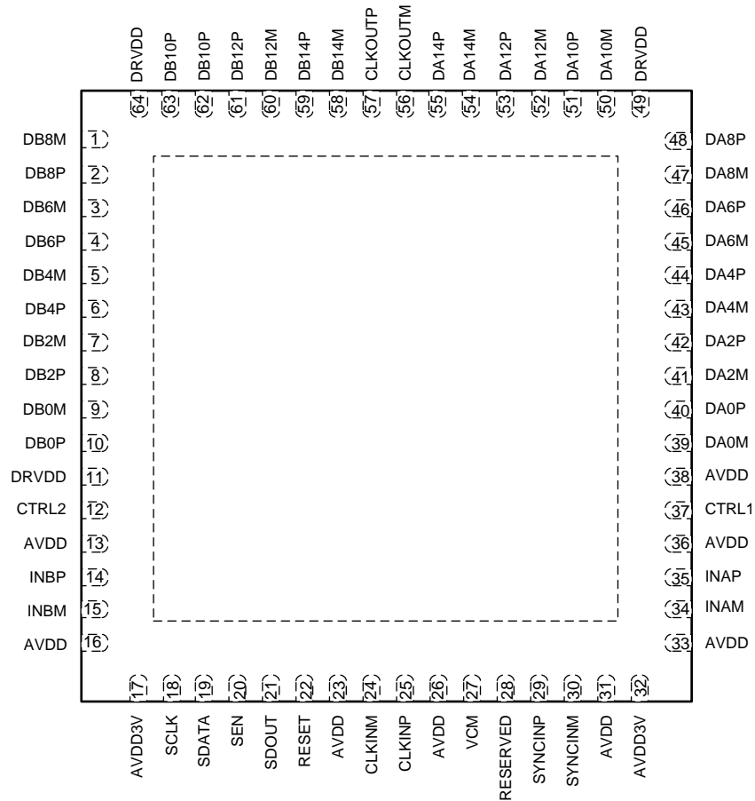
ADS42LB69 DDR LVDS: RGC Package VQFN-64 (Top View)
