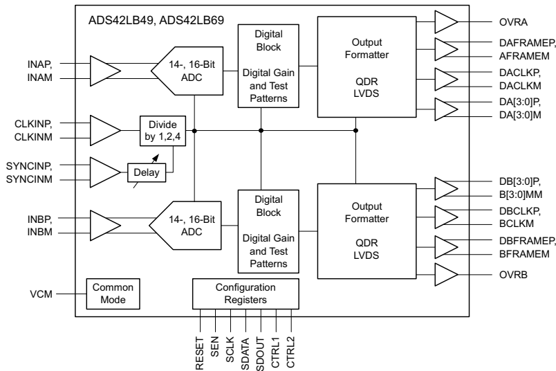
Figure 78. ADS42LB69, ADS42LB49 QDR LVDS
