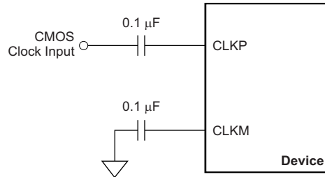
Figure 119. Single-Ended Clock Driving Circuit
