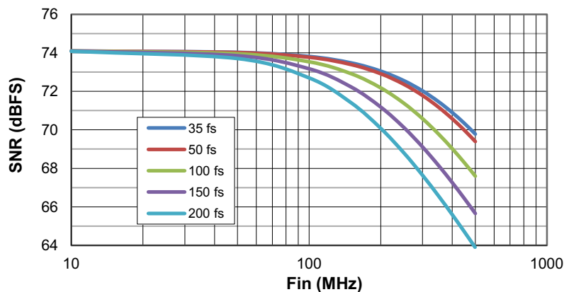
Figure 120. SNR versus Input Frequency and External Clock Jitter
