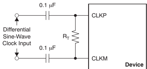
Figure 115. Differential Sine-Wave Clock Driving Circuit
