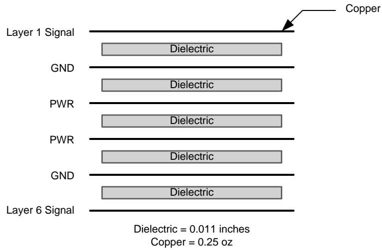
Figure 126. Example PCB Layer Stack
