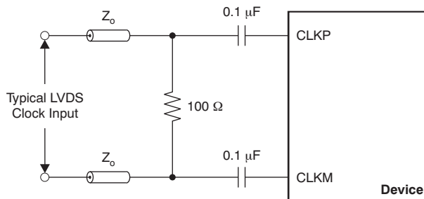
Figure 116. LVDS Clock Driving Circuit
