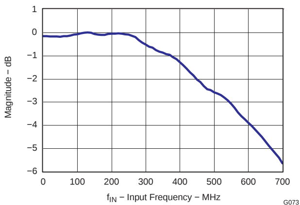
Figure 80. Analog Input Bandwidth
