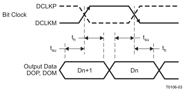
Figure 2. LVDS Timings
