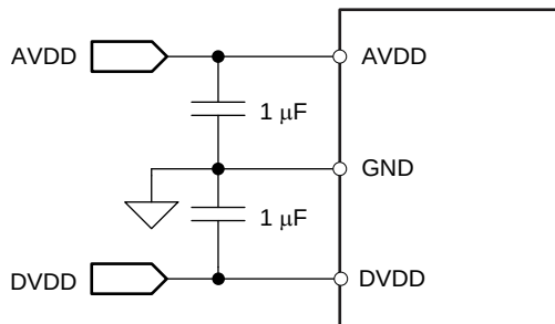
Figure 45. Power-Supply Decoupling
