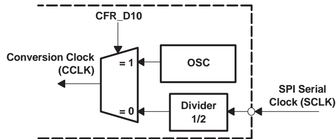
Figure 54. Converter Clock
