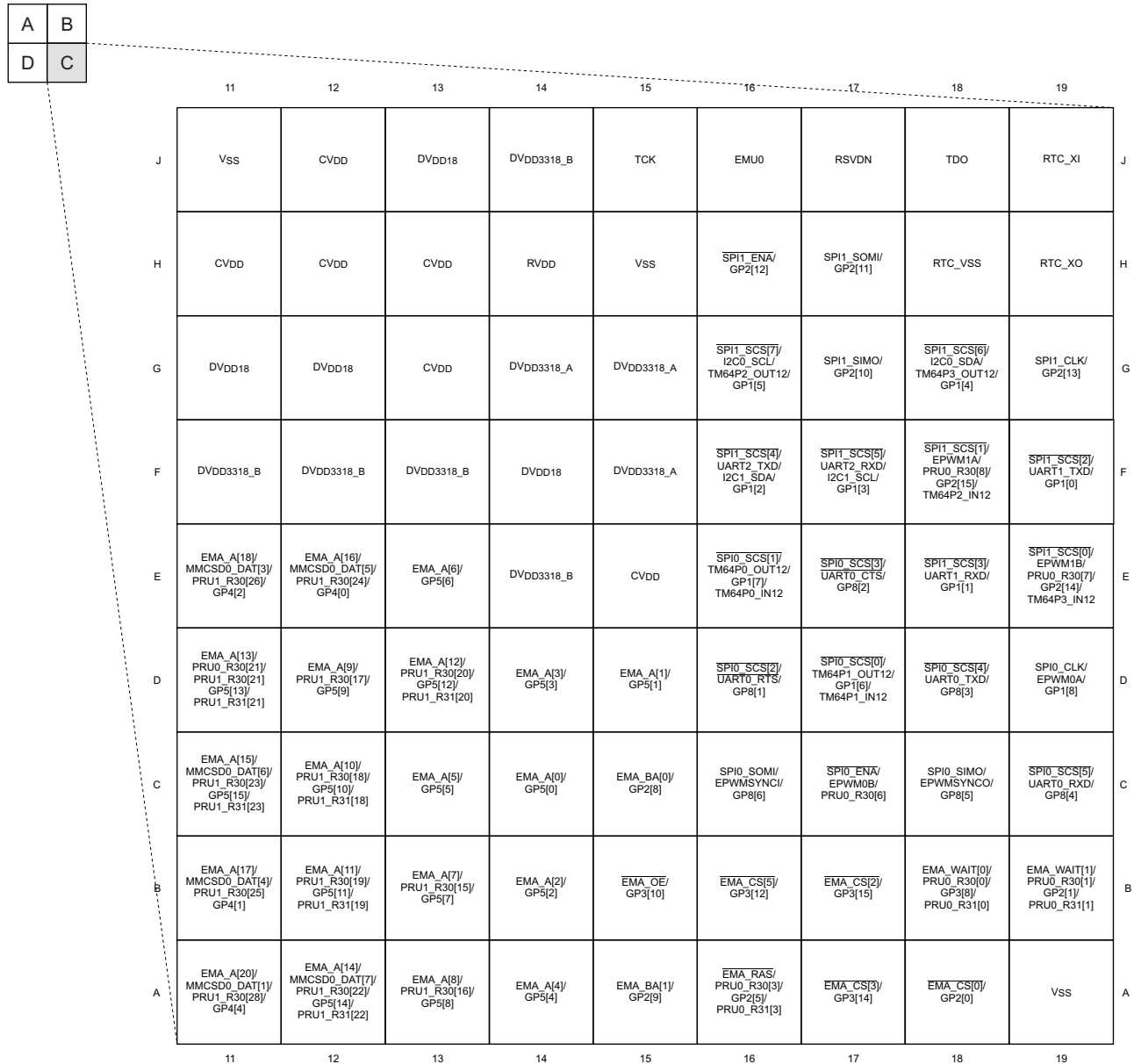
Figure 2-3. Pin Map (Quad C)
