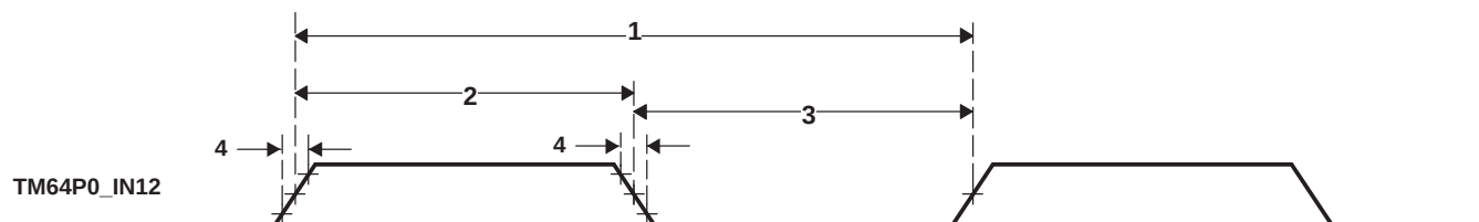
Figure 5-72. Timer Timing
