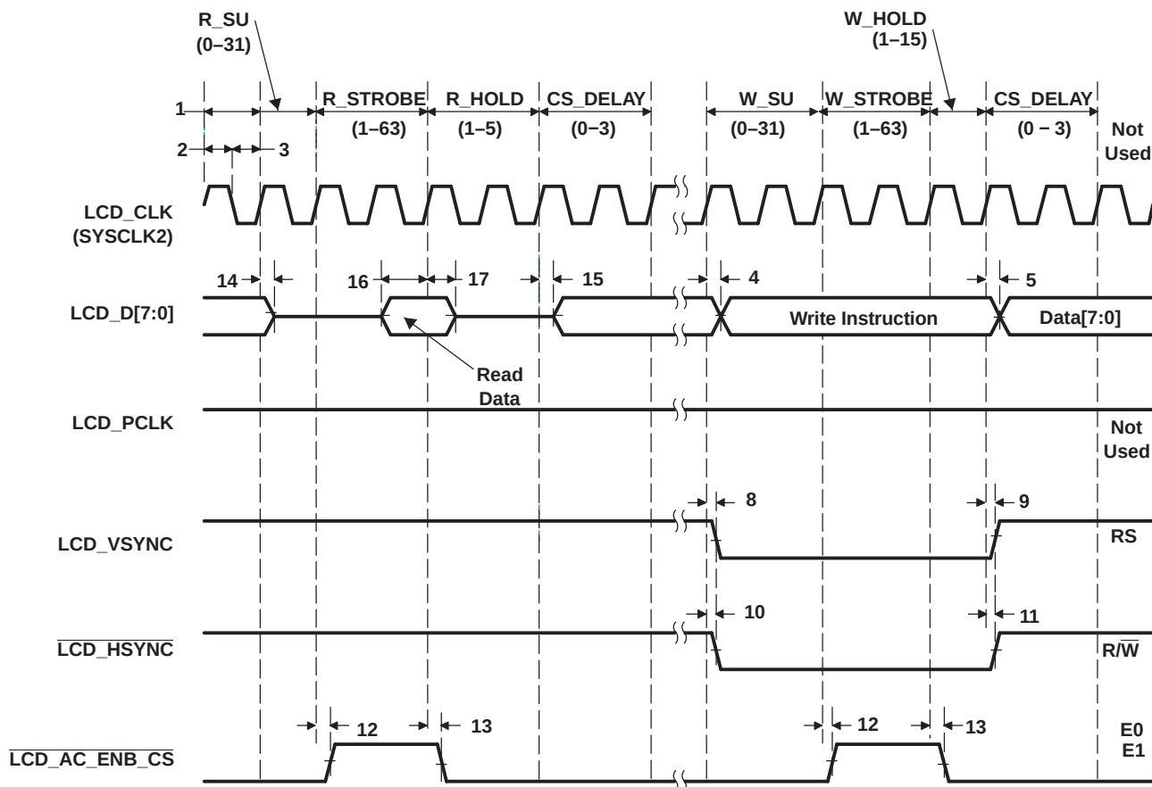
Figure 5-45. Character Display HD44780 Read
