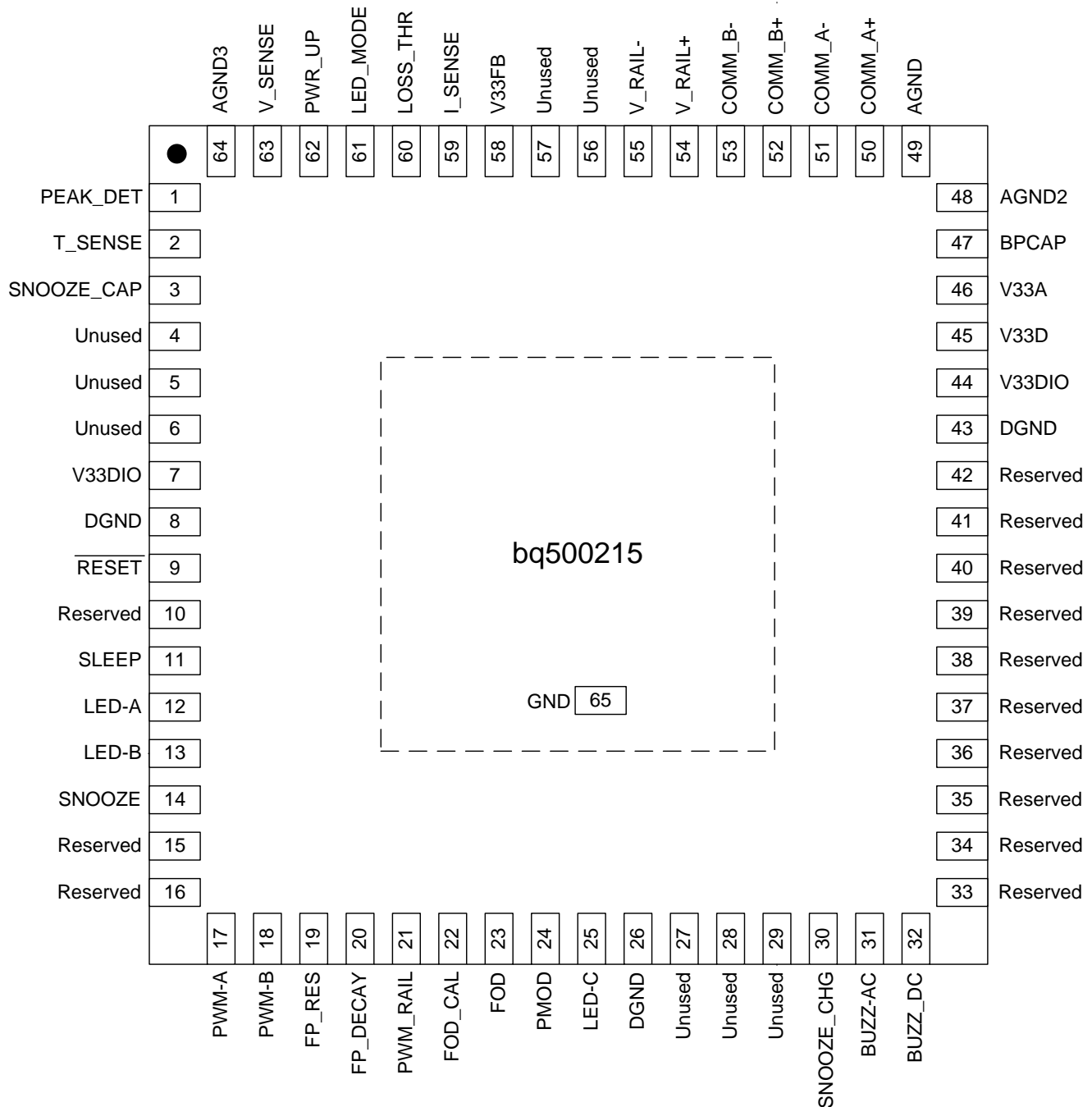
RGC (VQFN) PACKAGE (TOP VIEW)
