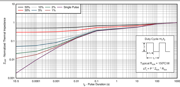
Figure 1. Transient Thermal Impedance
