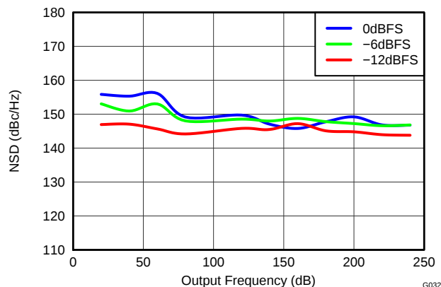
Figure 33. DAC3161 NSD vs Output Frequency Over Input Scale
