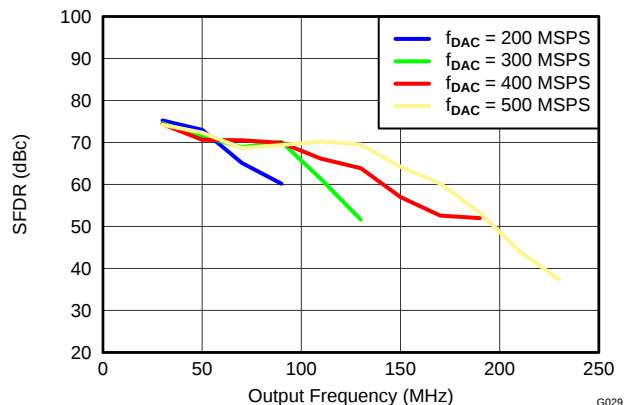
Figure 30. DAC3161 SFDR vs Output Frequency Over f_{DAC}
