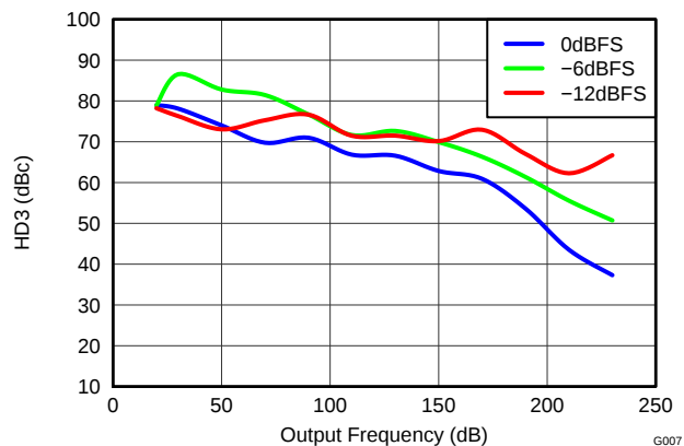
Figure 9. DAC3151 Third-Order Harmonic Distortion vs Output Frequency Over Input Scale
