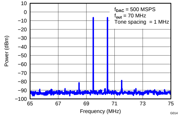
Figure 60. DAC3171 Two-Tone Spectral Plot (IF = 70MHz)
