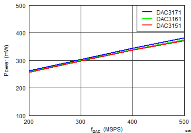
Figure 65. Power Consumption vs f_{\text{DAC}}
