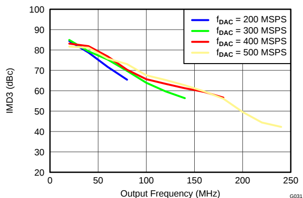
Figure 32. DAC3161 IMD3 vs Output Frequency Over f_{DAC}
