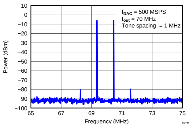
Figure 40. DAC3161 Two-Tone Spectral Plot (IF = 70MHz)
