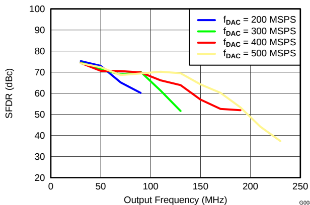
Figure 10. DAC3151 SFDR vs Output Frequency Over f_{DAC}
