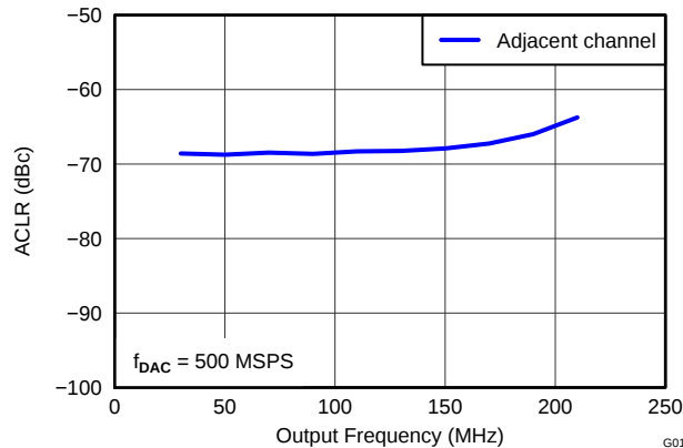
Figure 15. DAC3151 ACLR (Adjacent Channel) vs Output Frequency
