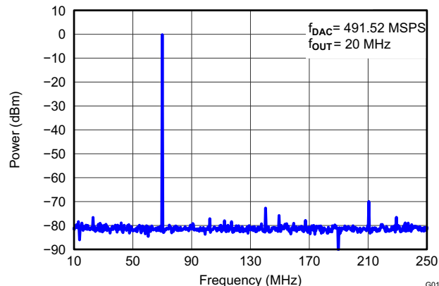
Figure 58. DAC3171 Single-Tone Spectral Plot (IF = 70MHz)
