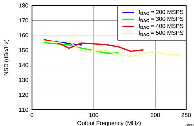
Figure 34. DAC3161 NSD vs Output Frequency Over f_{DAC}
