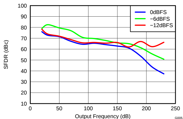
Figure 7. DAC3151 SFDR vs Output Frequency Over Input Scale
