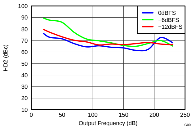
Figure 8. DAC3151 Second-Order Harmonic Distortion vs Output Frequency Over Input Scale
