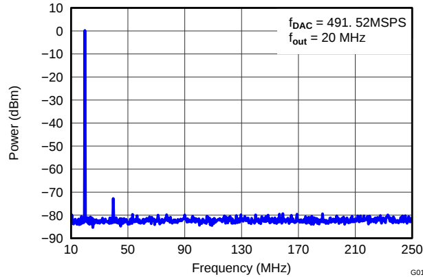
Figure 15. DAC3154 Single-Tone Spectral Plot (IF = 20MHz)
