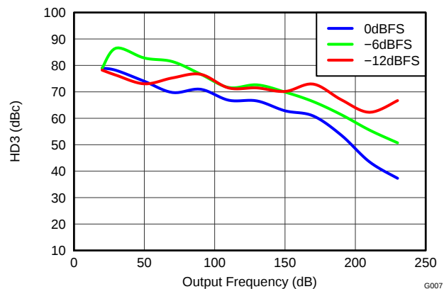
Figure 7. DAC3154 Third-Order Harmonic Distortion vs Output Frequency Over Input Scale
