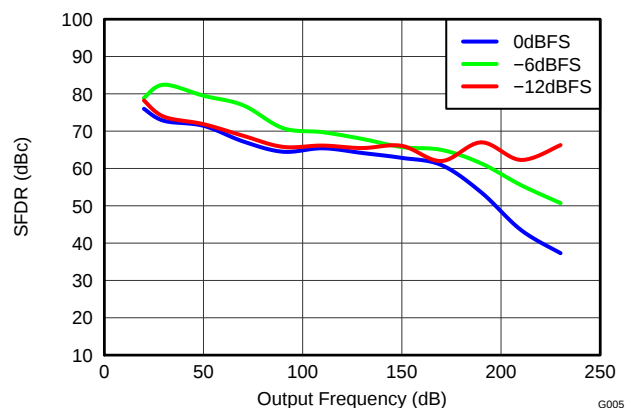
Figure 5. DAC3154 SFDR vs Output Frequency Over Input Scale
