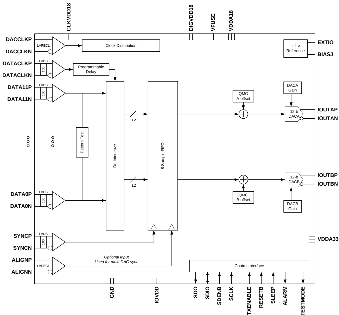
Figure 2. DAC3164
