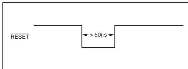
Figure 9. Reset Timing
