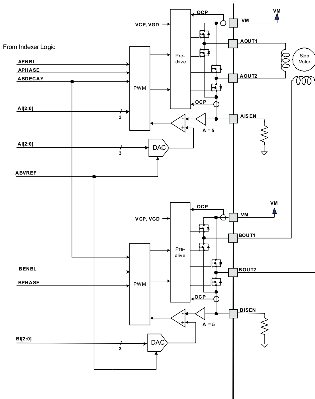
Figure 2. Block Diagram
