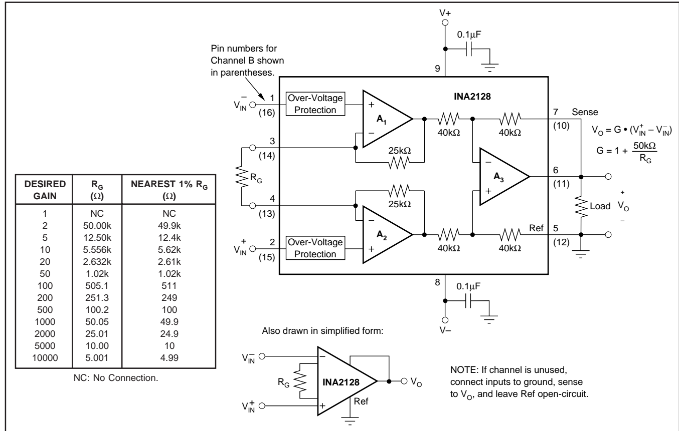
FIGURE 1. Basic Connections.
