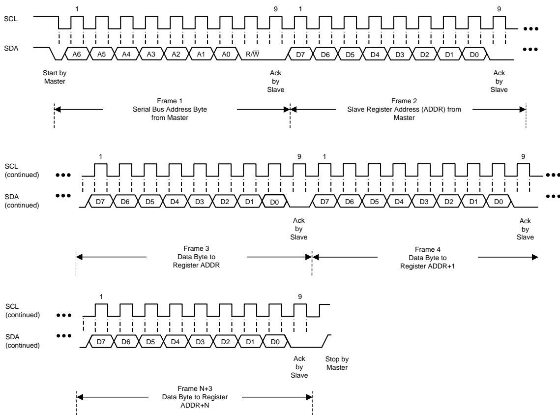
Figure 14. I 2 C Sequence of Writing Consecutive Registers
