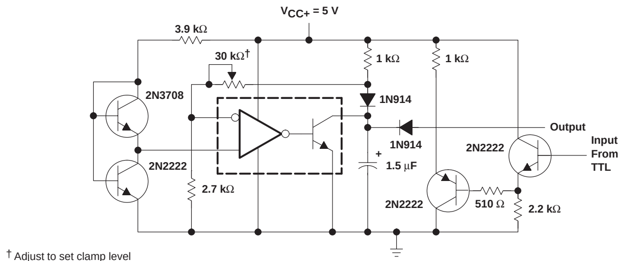
Figure 22. Precision Squarer
