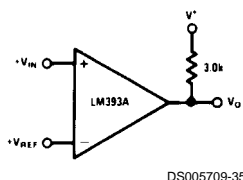
Basic Comparator
