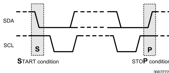
FIGURE 7. I 2 C Start and Stop Conditions
