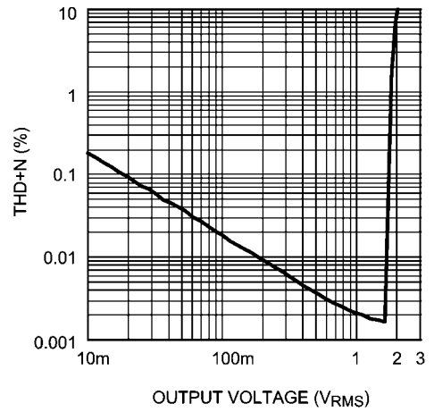
Auxiliary Output THD+N vs Output Voltage MONO/AUX Input, MONO/AUX Gain = 0dB, EP Gain = 0dB AVDD = 3.3V, f_{IN} = 1kHz , R_L = 5k\Omega AUXOUT Mode
