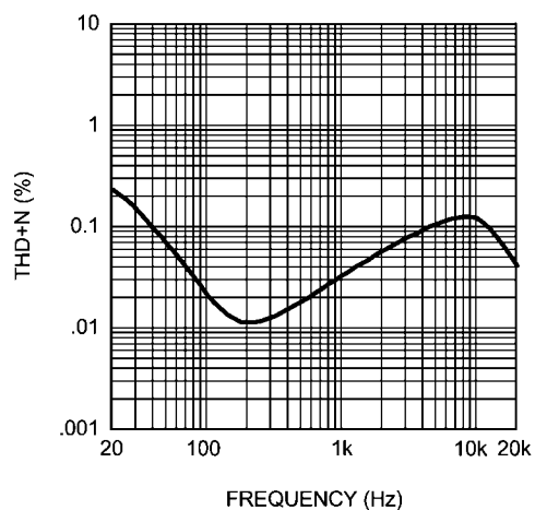
Earpiece THD+N vs Frequency MONO/AUX Input, MONO/AUX Gain = 0dB, EP Gain = 0dB AVDD = 3.3V, P_{OUT} = 20mW , R_L = 32\Omega Earpiece Mode
