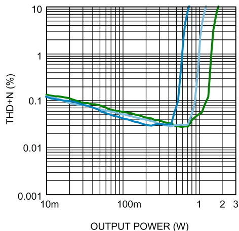
Loudspeaker THD+N vs Output Power From MONO/AUX Input, MONO/AUX Gain = 0dB LS Gain = 8dB, f_{IN} = 1kHz , R_L = 8\Omega Blue >> LSVDD = 3.3V Light Blue >> LSVDD = 4.2V Green >> LSVDD = 5V
