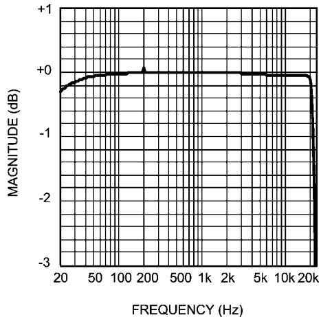
Stereo Audio ADC Frequency Response f_s = 48\text{kHz} , \text{OSR} = 64 From MIC, MIC Gain = 6dB, C_{IN} = 1\mu\text{F}
