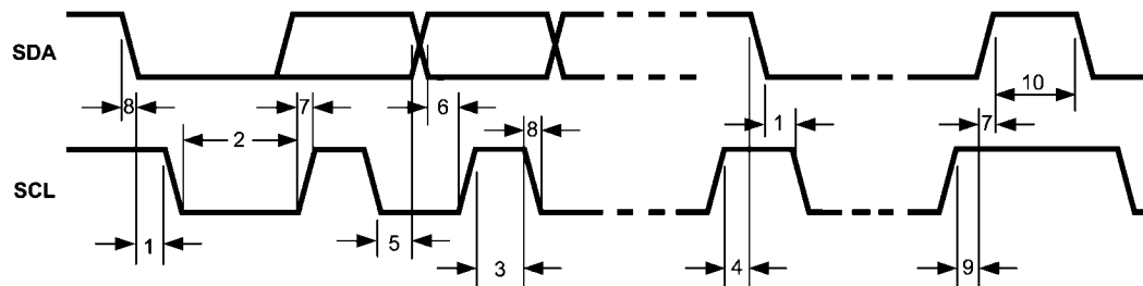
FIGURE 11. I²C Timing Diagram
