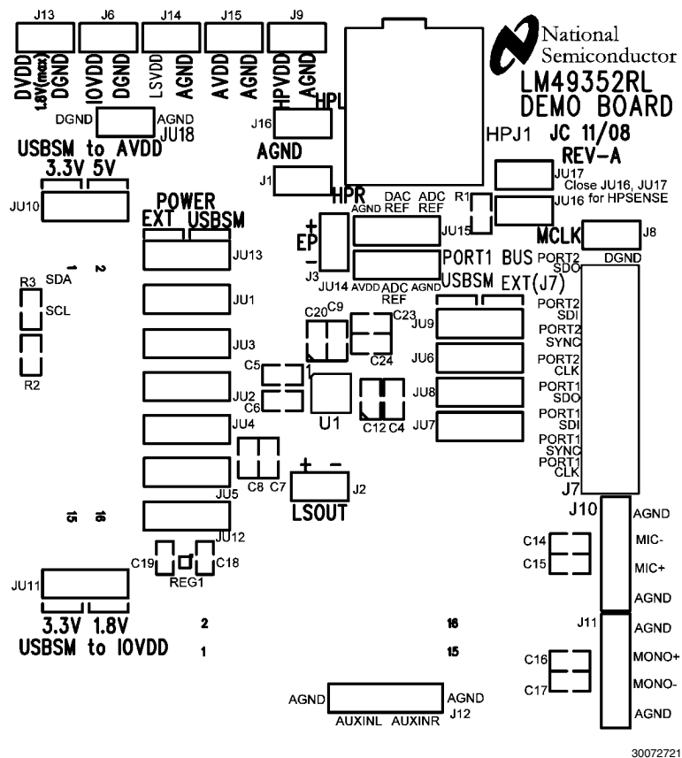
FIGURE 28. Top Silkscreen
