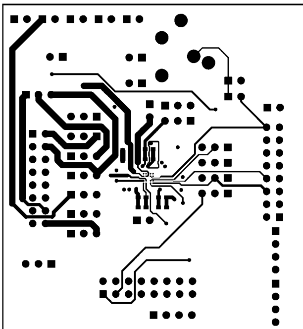
FIGURE 32. Bottom Layer
