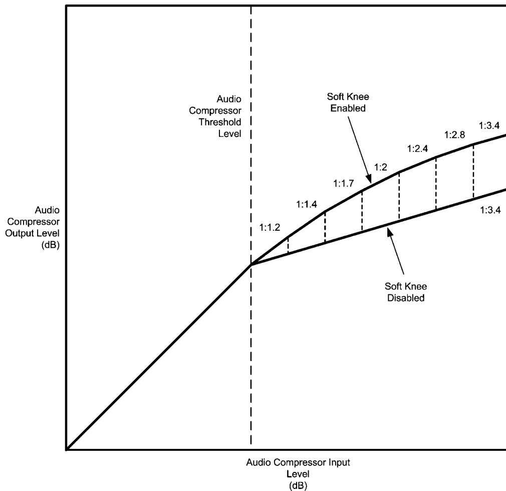
FIGURE 26. Soft Knee Example with Compression Ratio Setting of 1:3.4
