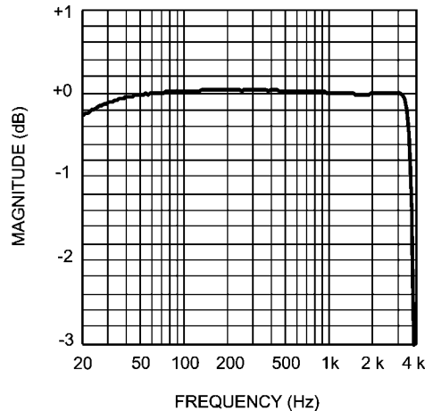
Stereo Audio ADC Frequency Response f_s = 8\text{kHz} , \text{OSR} = 128 From MIC, MIC Gain = 6dB, C_{IN} = 1\mu\text{F}
