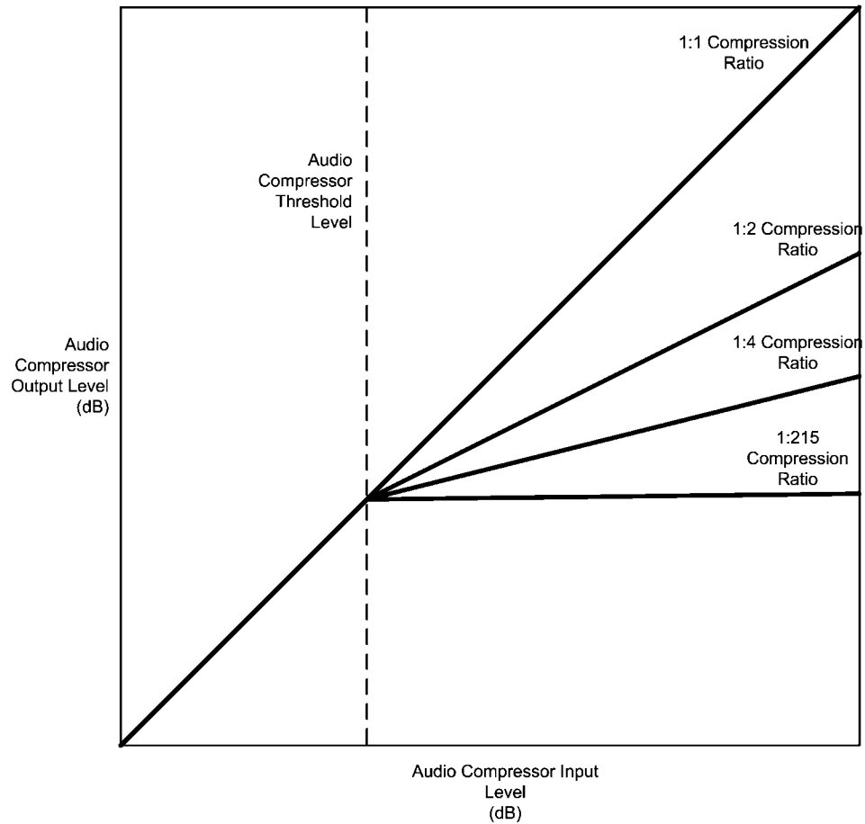
FIGURE 25. Audio Compressor Effect
