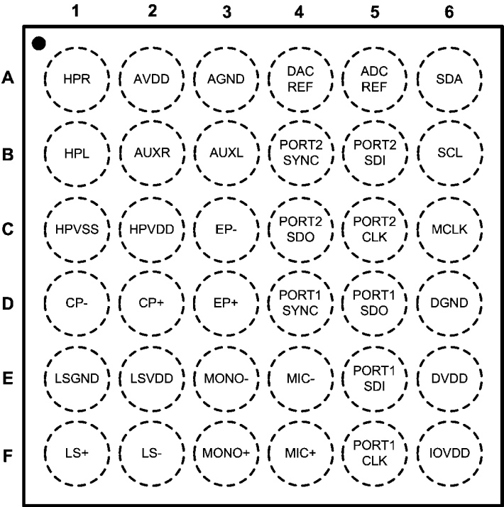
Top View (Bump Side Down)
