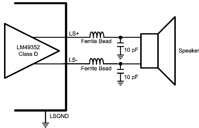
FIGURE 14. EMI/RFI Filter for the Class D Amplifier
