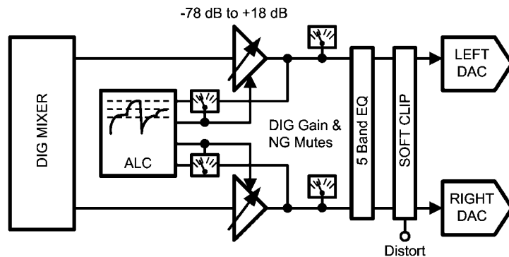
FIGURE 22. DAC DSP Effects Chain
