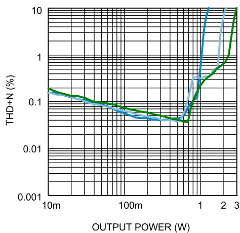
Loudspeaker THD+N vs Output Power f_S = 48kHz , OSR = 128 From MONO/AUX Input, MONO/AUX Gain = 0dB LS Gain = 8dB, f_{IN} = 1kHz , R_L = 4\Omega Blue >> LSVDD = 3.3V Light Blue >> LSVDD = 4.2V Green >> LSVDD = 5V
