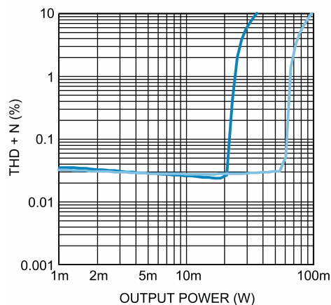
Headphone THD+N vs Output Power MONO/AUX Input, MONO/AUX Gain = 0dB, HP Gain = 0dB Stereo In Phase, f_{IN} = 1kHz , R_L = 32\Omega Blue >> HPVDD = 1.8V Light Blue >> HPVDD = 2.8V
