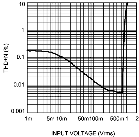
ADC THD+N vs Input Voltage f_s = 48\text{kHz} , \text{OSR} = 128 From MIC, MIC Gain = 6dB, V_{IN} = 1\text{kHz}
