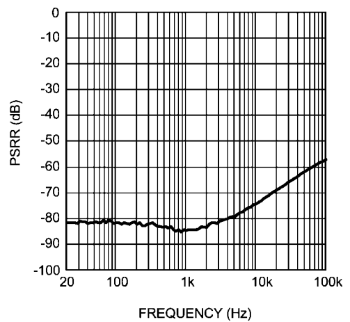
Headphone PSRR vs Frequency DAC Input, DAC Gain = 0dB, HP Gain = 0dB HPVDD = 1.8V, AVDD = 3.3V, DVDD = 1.8V, V_{RIPPLE} = 200\text{mV}_{PP} Ripple on HPVDD, AVDD, DVDD
