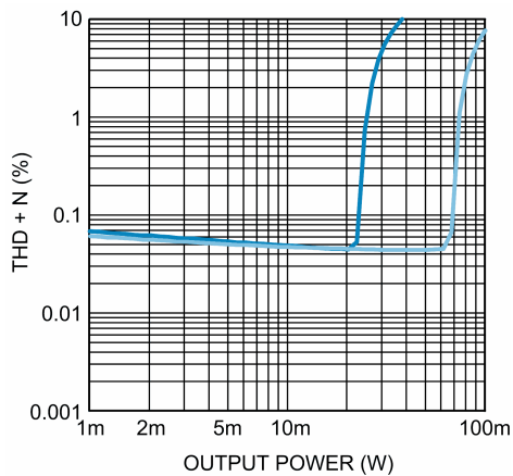
Headphone THD+N vs Output Power MONO/AUX Input, MONO/AUX Gain = 0dB, HP Gain = 0dB Stereo In Phase, f_{IN} = 1\text{kHz} , R_L = 16\Omega Blue >> HPVDD = 1.8V Light Blue >> HPVDD = 2.8V
