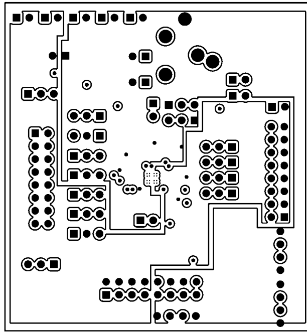
FIGURE 30. Inner Layer 2
