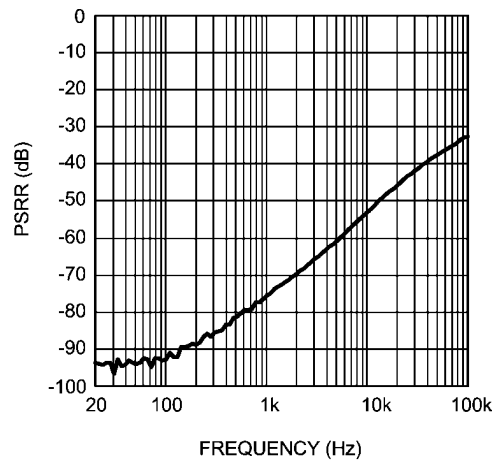
Headphone PSRR vs Frequency MONO/AUX Input, MONO/AUX Gain = 0dB, HP Gain = 0dB HPVDD = 1.8V, AVDD = 3.3V, V_{RIPPLE} = 200\text{mV}_{PP} Ripple on HPVDD, AVDD
