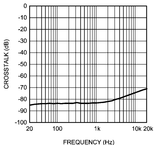
Headphone Crosstalk vs Frequency MONO/AUX Input, MONO/AUX Gain = 0dB, HP Gain = 0dB HPVDD = 1.8V, AVDD = 3.3V, P_{OUT} = 15mW , R_L = 32\Omega
