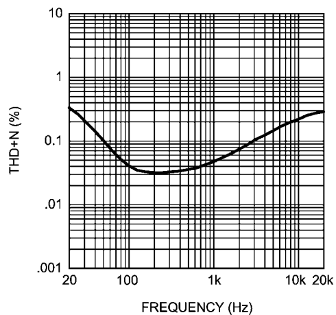
Headphone THD+N vs Frequency MONO/AUX, MONO/AUX Gain = 0dB, HP Gain = 0dB HPVDD = 1.8V, P_{OUT} = 15mW , R_L = 16\Omega Stereo In Phase
