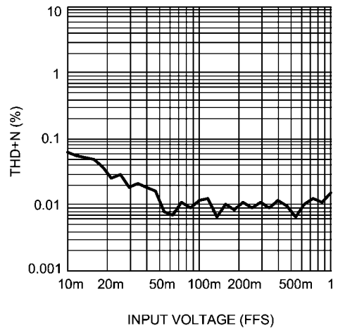
DAC THD+N vs Input Level f_s = 48\text{kHz} , \text{OSR} = 64 I^2S Input = 1kHz
