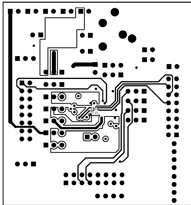
FIGURE 31. Inner Layer 3
