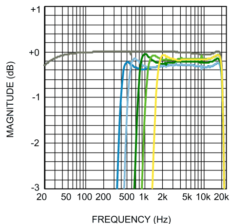
Mono Voice HPF ADC Frequency Response f_s = 48\text{kHz} , \text{OSR} = 128 From MIC, MIC Gain = 6dB, C_{IN} = 1\mu\text{F} Gray >> No HPF Blue >> HPF Mode = '000' Light Blue >> HPF Mode = '001' Green >> HPF Mode = '010' Light Green >> HPF Mode = '011' Yellow >> HPF Mode = '100'
