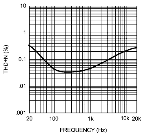
Headphone THD+N vs Frequency MONO/AUX, MONO/AUX Gain = 0dB, HP Gain = 0dB HPVDD = 2.8V, P_{OUT} = 15mW , R_L = 16\Omega Stereo in Phase
