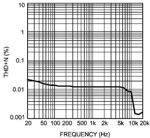
DAC THD+N vs Frequency f_s = 8\text{kHz} , \text{OSR} = 64 I^2S Input = 500mFFS
