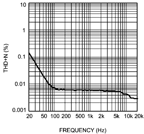
ADC THD+N vs Frequency f_s = 48\text{kHz} , \text{OSR} = 128 From MIC, MIC Gain = 6dB, V_{IN} = 500\text{mV}_{\text{RMS}}
