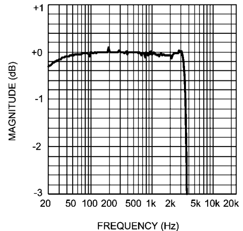
Mono Voice ADC Frequency Response f_s = 8\text{kHz} , \text{OSR} = 128 From MIC, MIC Gain = 6dB, C_{IN} = 1\mu\text{F}
