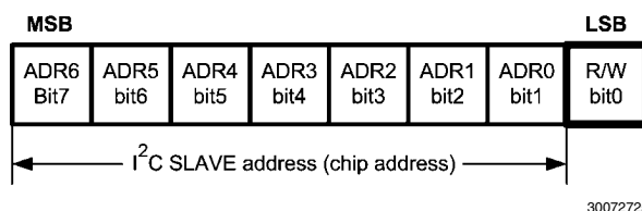
FIGURE 8. I 2 C Chip Address
