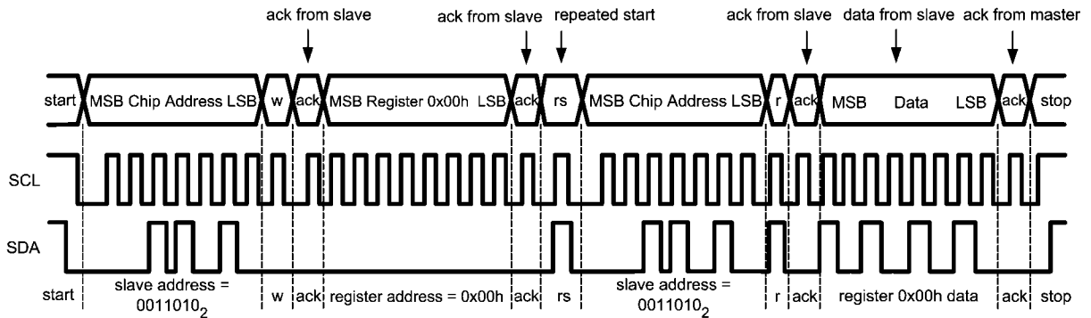
FIGURE 10. Example I²C Read Cycle
