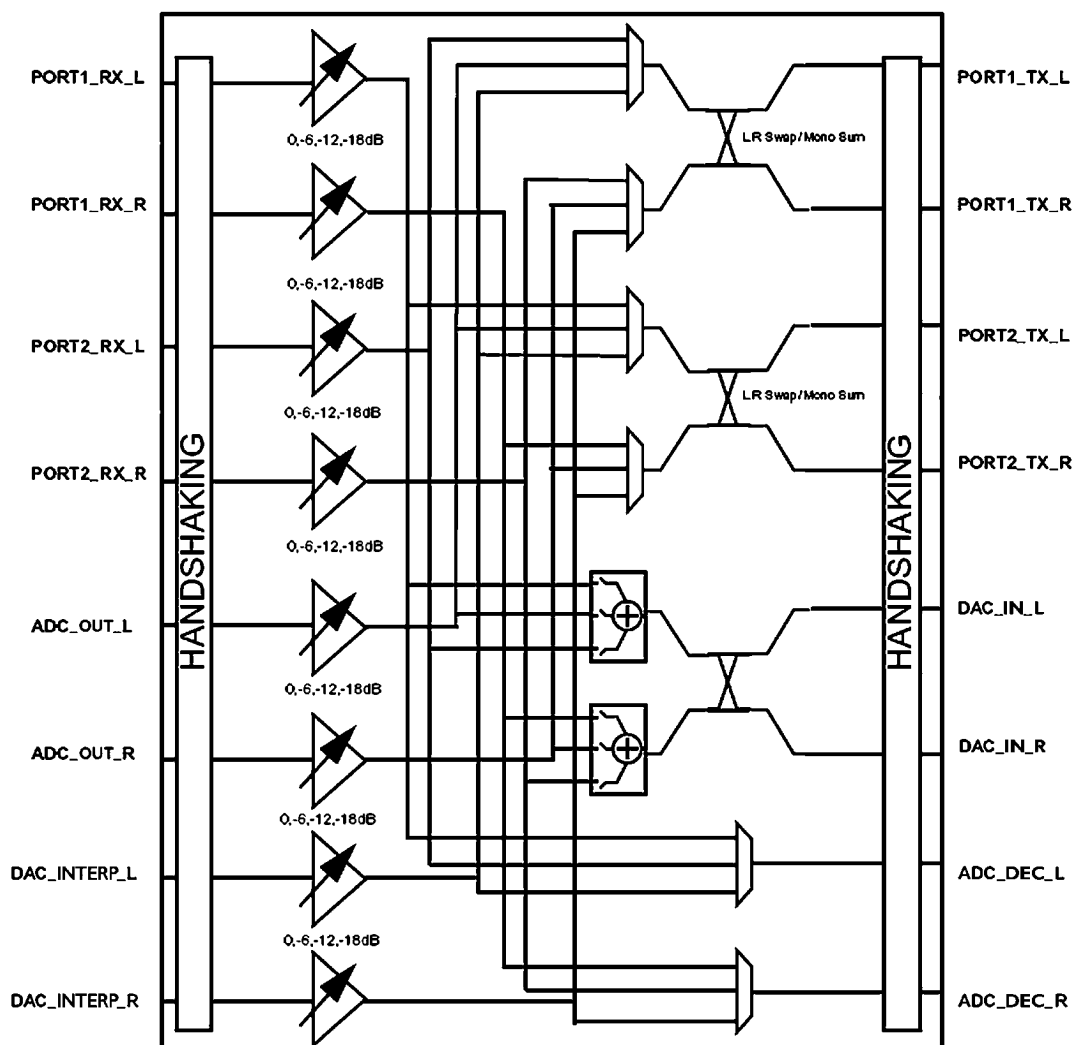
FIGURE 16. Digital Mixer
