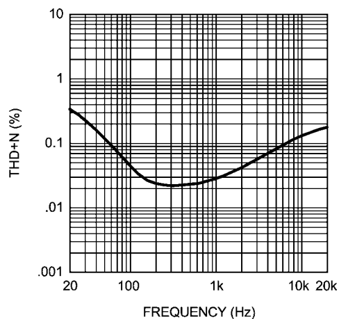
Headphone THD+N vs Frequency MONO/AUX, MONO/AUX Gain = 0dB, HP Gain = 0dB HPVDD = 2.8V, P_{OUT} = 15mW , R_L = 32\Omega Stereo In Phase
