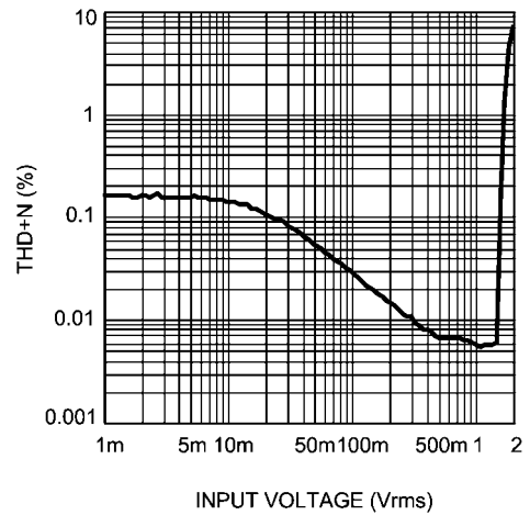
ADC THD+N vs Input Voltage f_s = 48\text{kHz} , \text{OSR} = 128 From MONO/AUX, MONO/AUX Gain = 0dB, f_{IN} = 1\text{kHz}
