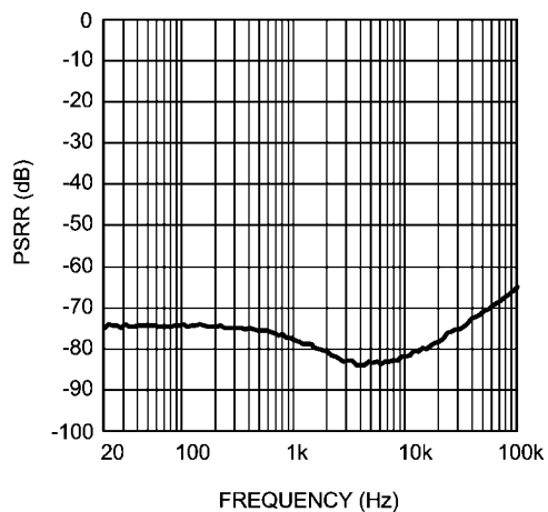
Loudspeaker PSRR vs Frequency f_s = 48\text{kHz} , \text{OSR} = 128 MONO/AUX Input, MONO/AUX Gain = 0dB, LS Gain = 12dB LSVDD = 4.2V, V_{\text{RIPPLE}} = 200\text{mV}_{\text{pp}} , Input Referred
