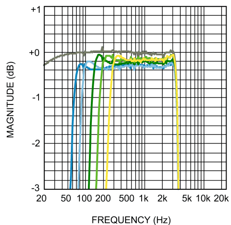
Mono Voice HPF ADC Frequency Response f_s = 8\text{kHz} , \text{OSR} = 128 From MIC, MIC Gain = 6dB, C_{IN} = 1\mu\text{F} Gray >> No HPF Blue >> HPF Mode = '000' Light Blue >> HPF Mode = '001' Green >> HPF Mode = '010' Light Green >> HPF Mode = '011' Yellow >> HPF Mode = '100'
