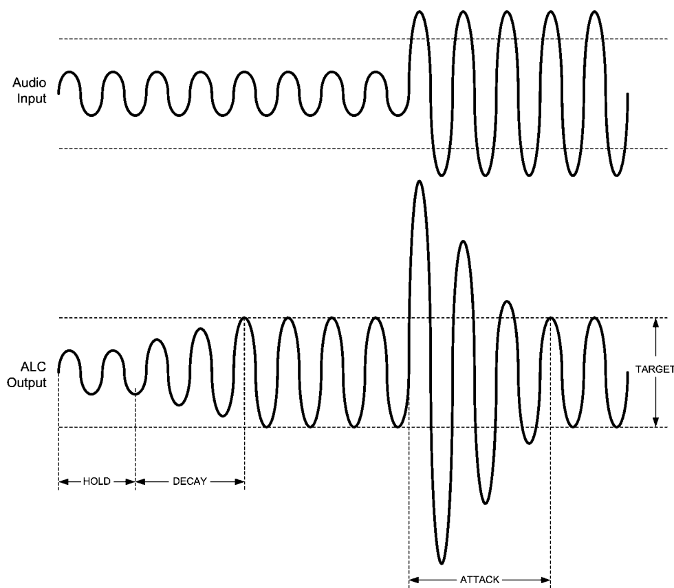
FIGURE 23. ALC Example
