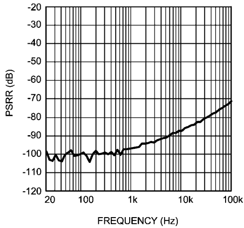
Auxiliary Output PSRR vs Frequency MONO/AUX Input, MONO/AUX Gain = 0dB, EP Gain = 0dB AVDD = 3.3V, V_{RIPPLE} = 200mV_{PP} , AUXOUT Mode
