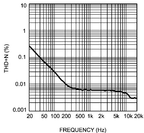
ADC THD+N vs Frequency f_s = 48\text{kHz} , \text{OSR} = 128 From MONO/AUX, MONO/AUX Gain = 6dB, V_{IN} = 1V_{RMS}
