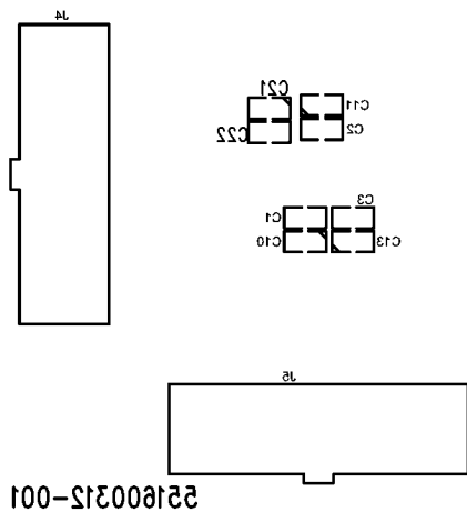
FIGURE 33. Bottom Silkscreen
