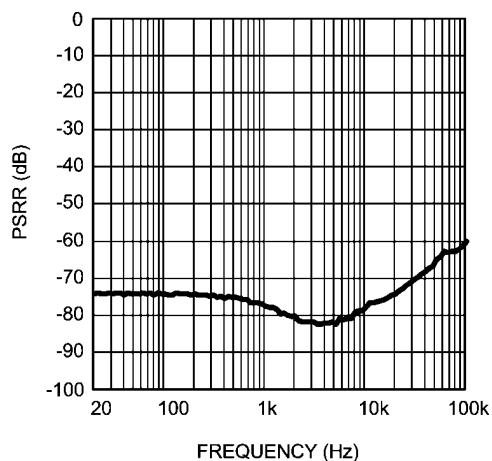
Loudspeaker PSRR vs Frequency MONO/AUX Input, MONO/AUX Gain = 0dB, LS Gain = 12dB LSVDD = 3.3V, V_{RIPPLE} = 200mV_{PP} , Input Referred
