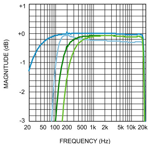
Stereo Audio HPF ADC Frequency Response f_s = 48\text{kHz} , \text{OSR} = 128 From MONO/AUX, MONO>AUX Gain = 0dB, C_{IN} = 1\mu\text{F} Blue >> No HPF Light Blue >> HPF Mode = '101' Green >> HPF Mode = '110' Light Green >> HPF Mode = '111'
