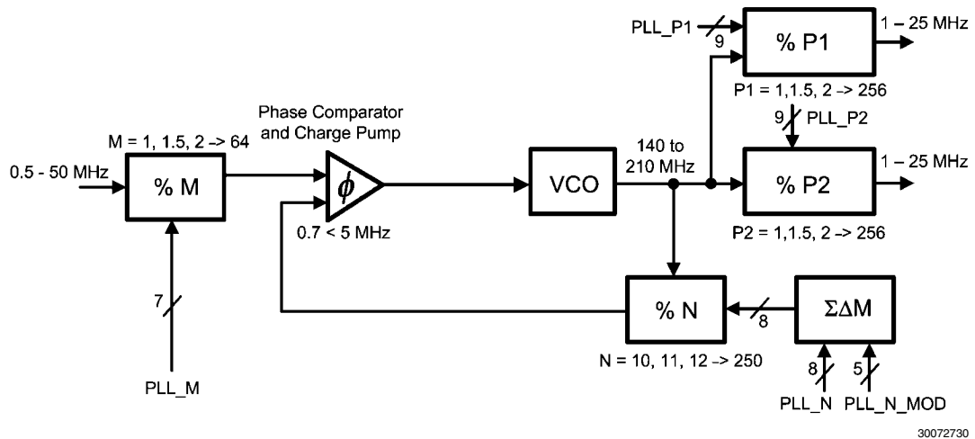
FIGURE 13. PLL Loop
