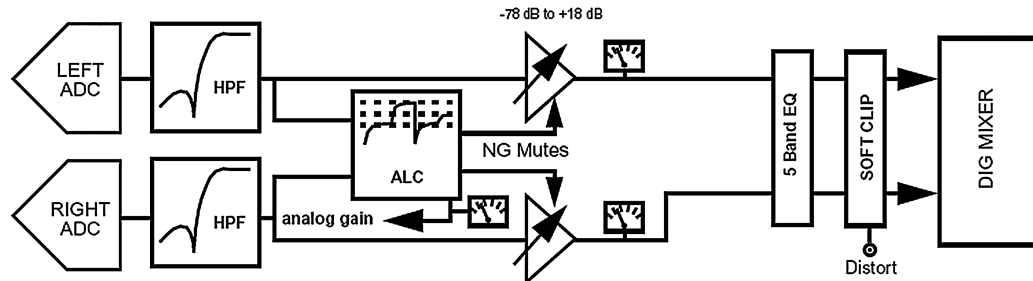
FIGURE 21. ADC DSP Effects Chain
