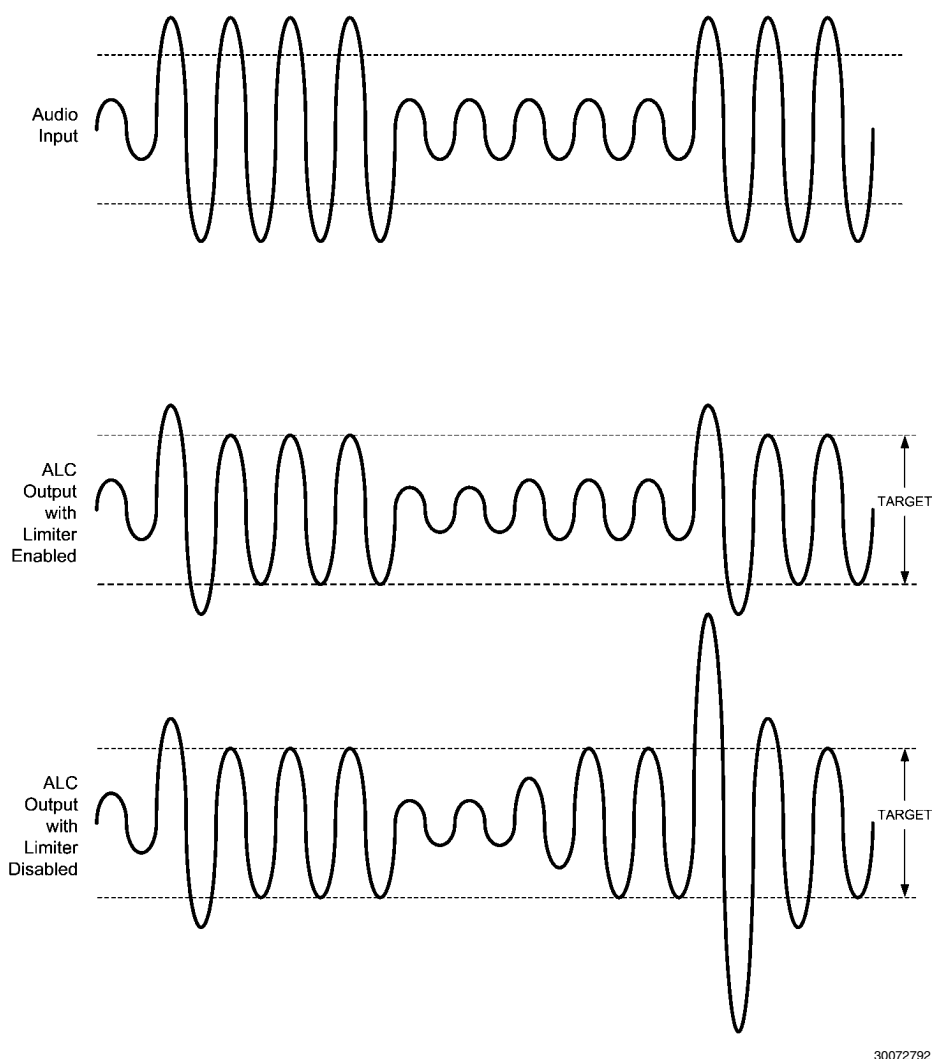
FIGURE 24. ALC Limiter
