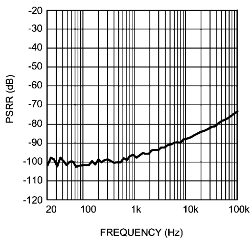
Earpiece PSRR vs Frequency MONO/AUX Input, MONO/AUX Gain = 0dB, EP Gain = -6dB AVDD = 3.3V, V_{RIPPLE} = 200mV_{PP} , Earpiece Mode
