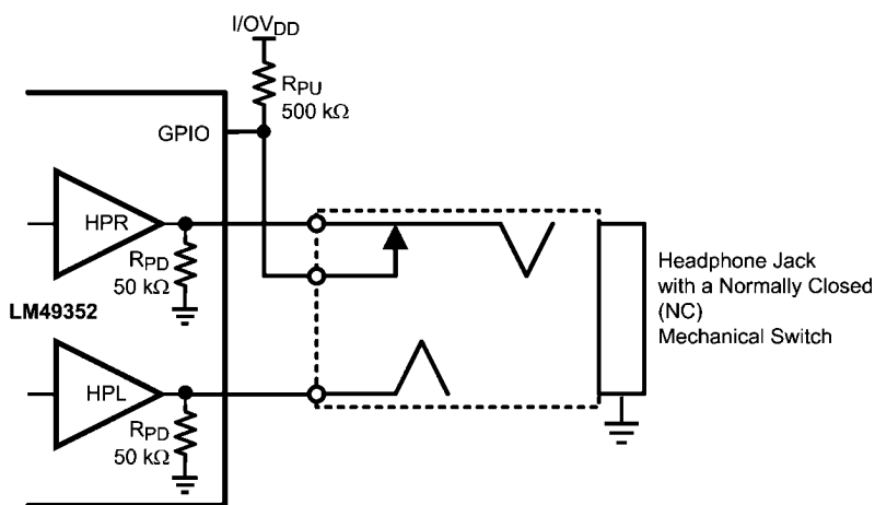
FIGURE 15. Application Circuit for Headphone Detection
