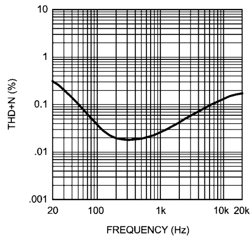
Headphone THD+N vs Frequency MONO/AUX, MONO/AUX Gain = 0dB, HP Gain = 0dB HPVDD = 3.3V, P_{\text{OUT}} = 15\text{mW} , R_L = 32\Omega Stereo In Phase
