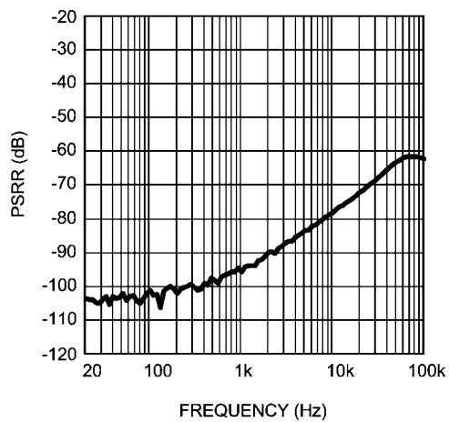
Headphone PSRR vs Frequency MONO/AUX Input, MONO/AUX Gain = 0dB, HP Gain = 0dB HPVDD = 1.8V, AVDD = 3.3V, V_{RIPPLE} = 200\text{mV}_{PP} Ripple on AVDD only
