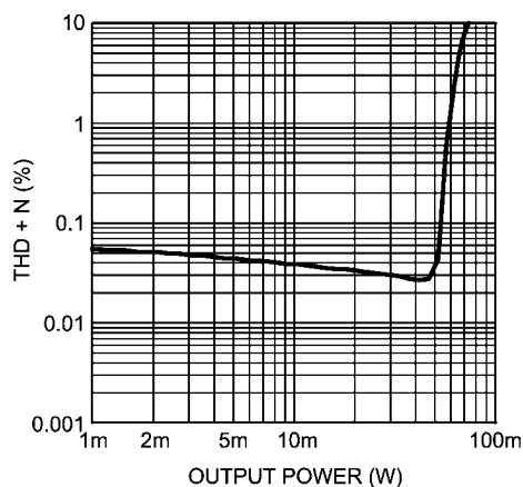
Earpiece THD+N vs Output Power MONO/AUX Input, MONO/AUX Gain = 0dB, EP Gain = 0dB AVDD = 3.3V, f_{IN} = 1kHz , R_L = 32\Omega Earpiece Mode
