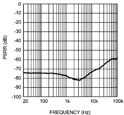
Loudspeaker PSRR vs Frequency MONO/AUX Input, MONO/AUX Gain = 0dB, LS Gain = 12dB LSVDD = 5V, V_{\text{RIPPLE}} = 200\text{mV}_{\text{pp}} , Input Referred
