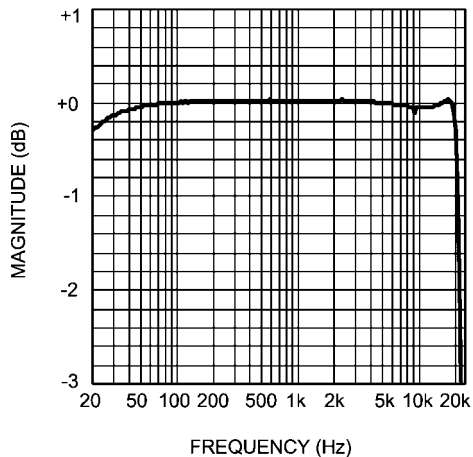
Mono Voice ADC Frequency Response f_s = 48\text{kHz} , \text{OSR} = 128 From MIC, MIC Gain = 6dB, C_{IN} = 1\mu\text{F}
