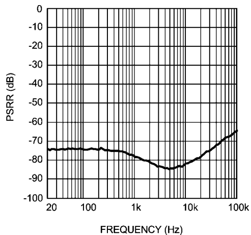
Headphone PSRR vs Frequency DAC Input, DAC Gain = 0dB, LS Gain = 12dB LSVDD = 3.3V, AVDD = 3.3V, DVDD = 1.8V, V_{\text{RIPPLE}} = 200\text{mV}_{\text{pp}} Ripple on LSVDD, AVDD, DVDD, Input Referred
