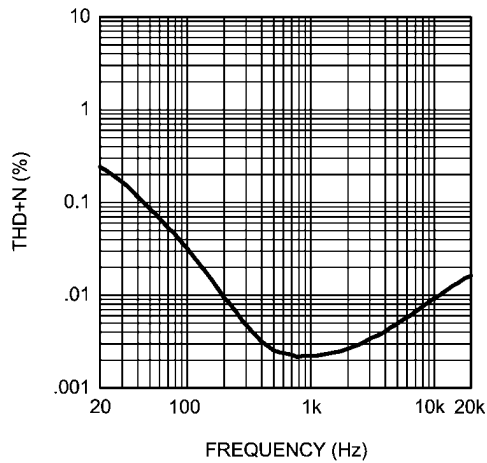
Auxiliary Output THD+N vs Frequency MONO/AUX Input, MONO/AUX Gain = 0dB, EP Gain = 0dB AVDD = 3.3V, V_{OUT} = 1V_{RMS} , R_L = 5k\Omega AUXOUT Mode
