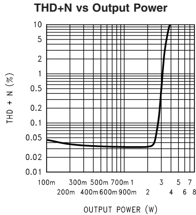
V_{DD} = 12V , R_L = 4\Omega , SE operation, both channels driven and loaded (average shown), f_{IN} = 1kHz
