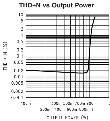
V_{DD} = 12V , R_L = 16\Omega , SE operation, both channels driven and loaded (average shown), f_{IN} = 1kHz
