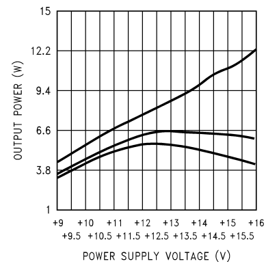
R_L = 8\Omega , BTL, f_{IN} = 1kHz , at (from top to bottom at 12V): THD+N = 10% THD+N = 1%, THD+N = 0.2%
