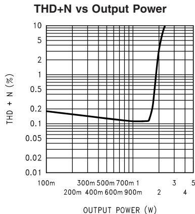
V_{DD} = 12V , R_L = 8\Omega , SE operation, A_V = 10 both channels driven and loaded (average shown), f_{IN} = 1kHz
