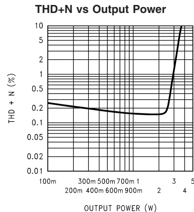
V_{DD} = 12V , R_L = 4\Omega , SE operation, A_V = 10 both channels driven and loaded (average shown), f_{IN} = 1kHz
