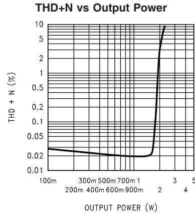
V_{DD} = 12V , R_L = 8\Omega , SE operation, both channels driven and loaded (average shown), f_{IN} = 1kHz
