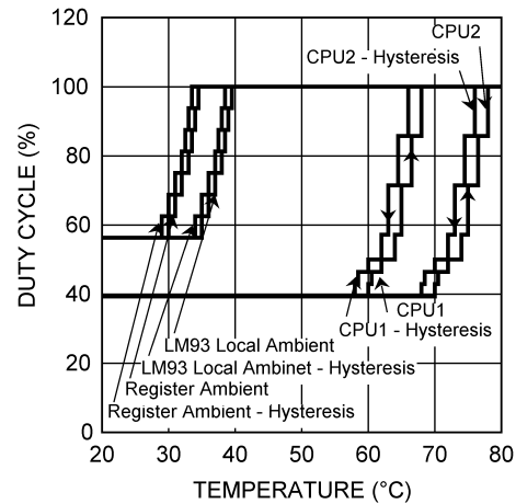
FIGURE 1. Example of the LM93 Fan Control Transfer Function. Download an excel spread sheet from www.national.com/appinfo/tempsensors that allows you to enter the fan control register values and then automatically generate a similar curve.
