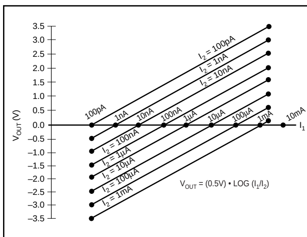
FIGURE 13. Transfer Function with Varying I_2 and I_1 .
