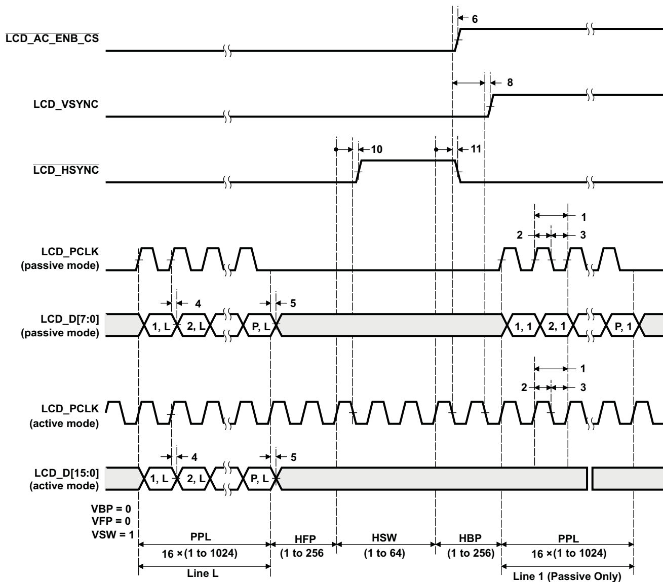
Figure 5-56. LCD Raster-Mode Control Signal Activation
