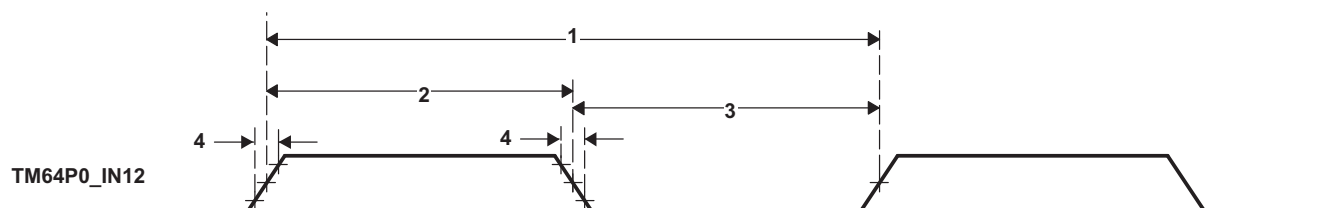
Figure 5-58. Timer Timing
