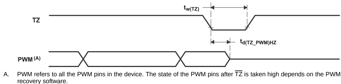
Figure 5-44. PWM Hi-Z Characteristics
