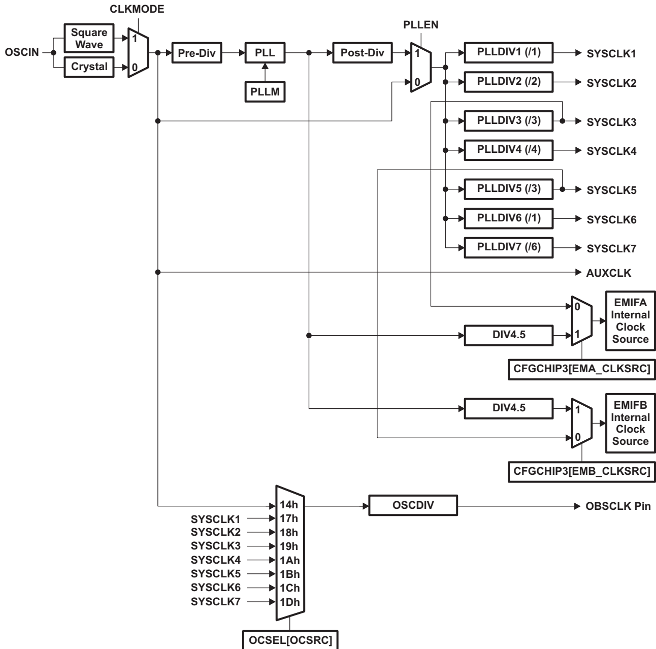
Figure 5-9. PLL Topology
