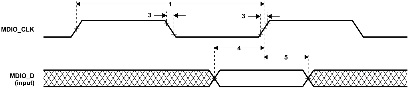
Figure 5-29. MDIO Input Timing
