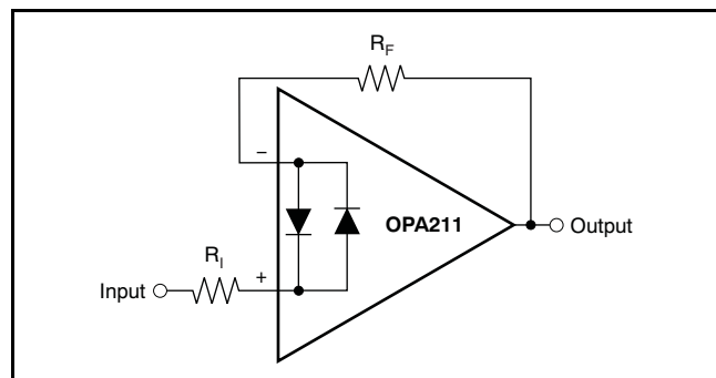
Figure 45. Pulsed Operation
