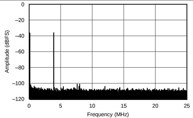
Figure 109. FFT for 450-MHz Input Signal, Dither Off
