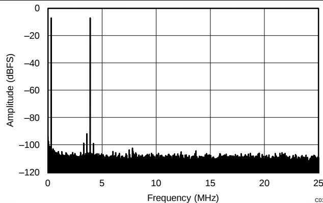
Figure 108. FFT for 450-MHz Input Signal, Dither On
