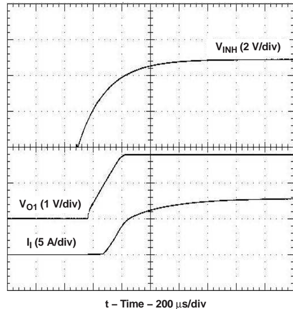
Figure 15. Power-Up Response from Inhibit Control
