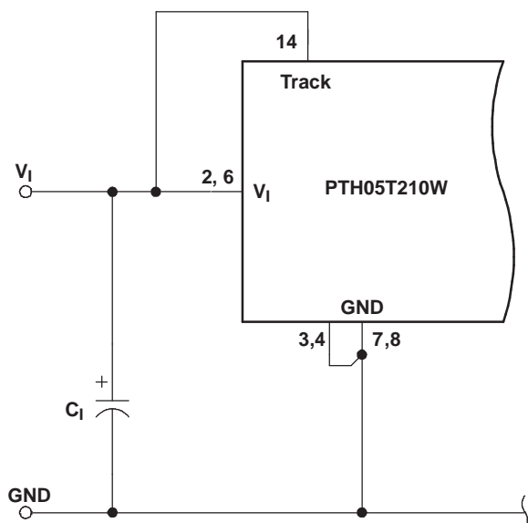
Figure 12. Power-Up Application Circuit
