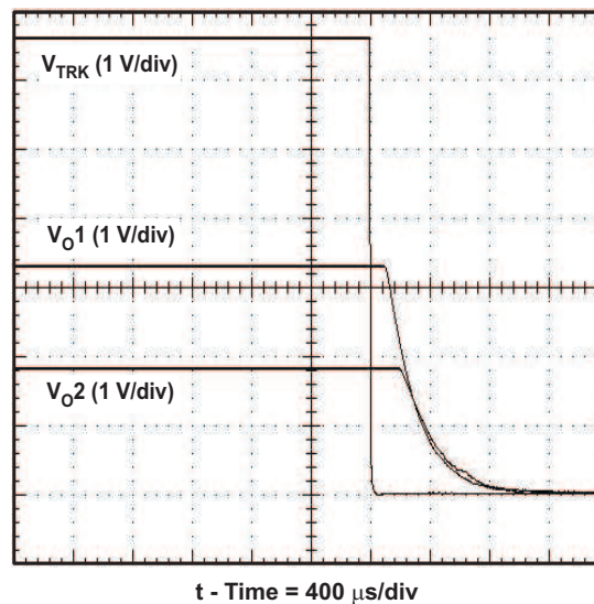
Figure 28. Simultaneous Power Down With Auto-Track Control
