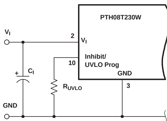
Figure 19. UVLO Implementation
