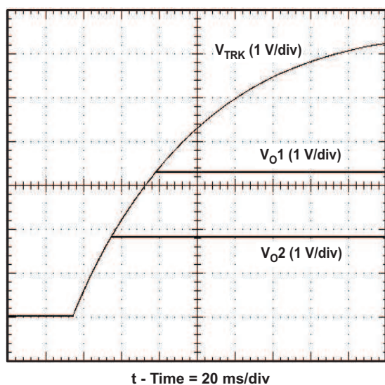
Figure 27. Simultaneous Power Up With Auto-Track Control
