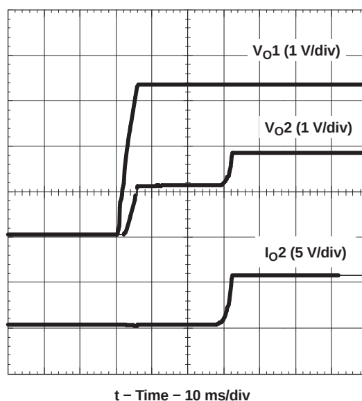
Figure 17. Prebias Startup Waveforms
