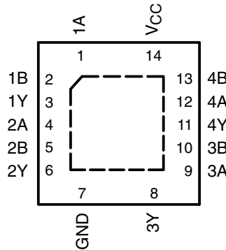
SN74AHC32 . . . RGY PACKAGE (TOP VIEW)
