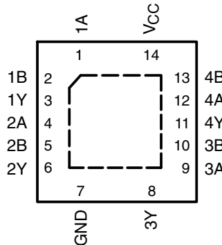
SN74AHC86 . . . RGY PACKAGE (TOP VIEW)
