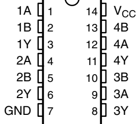
SN54AHC86 . . . J OR W PACKAGE SN74AHC86 . . . D, DB, DGV, N, NS, OR PW PACKAGE (TOP VIEW)
